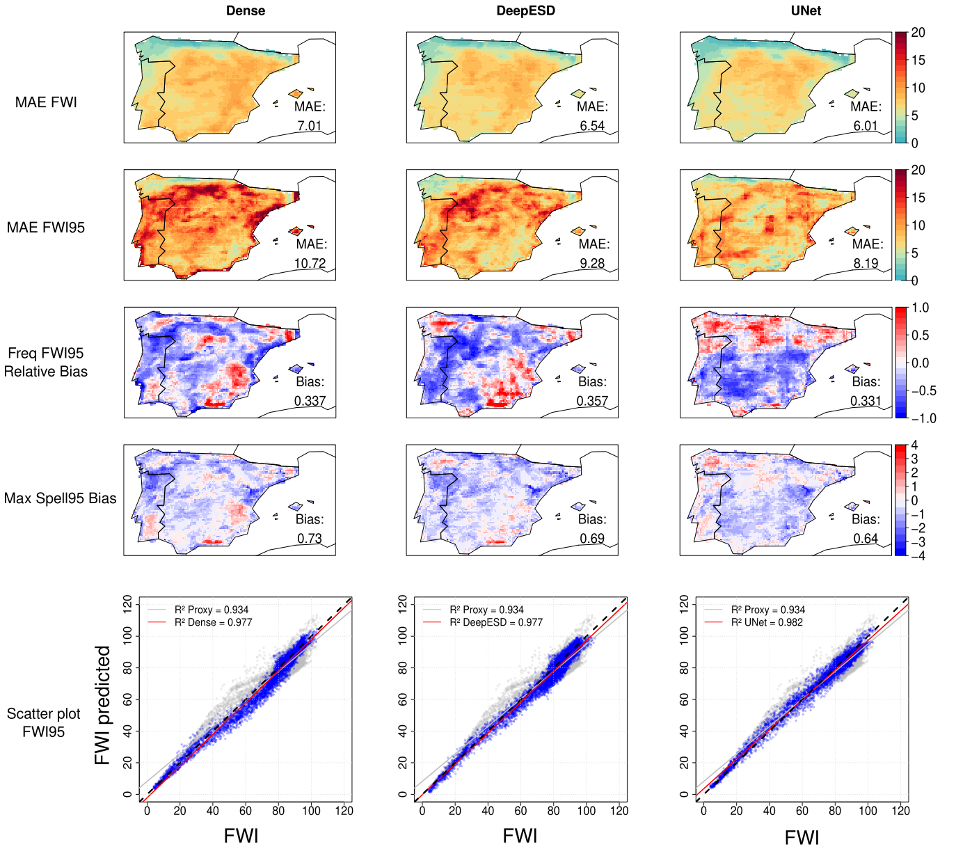
Figure 3. DL model results for various spatial validation indices presented in Figure 2. The results depict the differences relative to the reference FWI for the fire season (June–September) during the test period (2018–2021). The scatter plots compare climatology values between the Proxy FWI95 (in grey) and the corresponding DL model predictions (in blue), against reference FWI95. Linear fits are shown in grey for the Proxy FWI95 and in red for the DL model, with the corresponding R^2 values displayed in the top-left corner.
