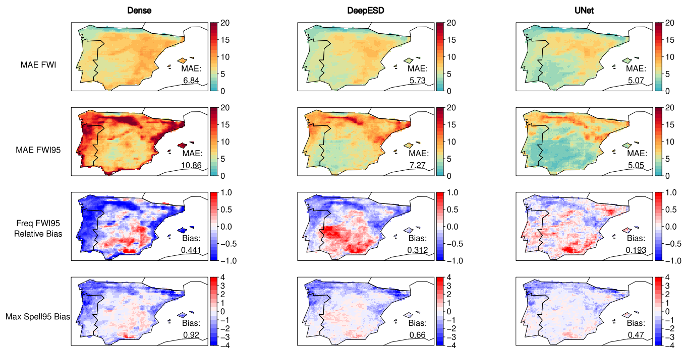
Figure D1. Results from the Dense, DeepESD and U-Net model trained with 12UTC input variables (temperature, 24h-accumulated precipitation, relative humidity and wind speed). The maps display differences relative to the reference FWI for the fire season (June–September) during the test period (2018–2021) for the validation indices. The MAE value inside the map represents the spatially aggregated mean absolute error of the deep learning predictions with respect to the FWI reference, while Bias denotes the spatially averaged bias in absolute value.
