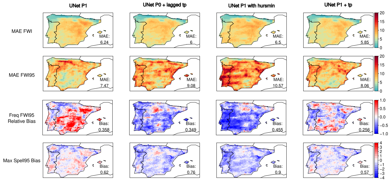
Figure D2. Results from the U-Net model trained with the P1 predictors set (see Table 1), trained with P0 and adding the 24-h lagged precipitation, trained with P1 adding minimum relative humidity instead of daily mean relative humidity and trained with P1 adding precipitation. The maps display differences relative to the reference FWI for the fire season (June–September) during the test period for different validation indices. MAE represents the spatially aggregated mean absolute error of the deep learning predictions with respect to the FWI reference, while Bias denotes the spatially averaged bias in absolute value.
