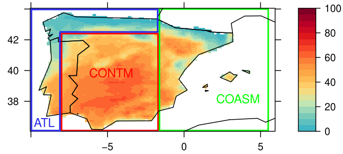
Figure A1. Climatological regions within the Iberian Peninsula used for XAI analysis in Figure 6. Blue, green and red rectangles indicate ATL (Atlantic), COASM (Coastal Mediterranean), and CONTM (Continental Mediterranean) regions respectively.
