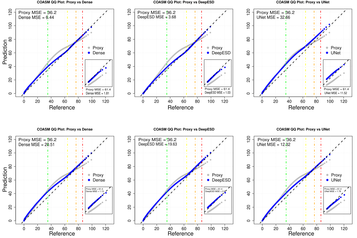
Figure C1. Quantile-Quantile (QQ) plots comparing the Proxy FWI (in grey) and DL model results (in blue). The results for the Coastal Mediterranean (COASM) (Figure A1 for the subregion boundaries). Dash-dotted vertical lines indicate different fire danger levels established by the Agencia Estatal de Meteorología (AEMET). Fire danger levels are defined as follows: low (below the green line), moderate (between the green and yellow lines), high (between the yellow and orange lines), very high (between the orange and red lines), and extreme (above the red line). The Mean Squared Error (MSE) for both results is displayed in the top right corner. A box in the bottom right provides an amplified view of QQ plot focused on values above the 95th percentile (extreme danger), along with the corresponding MSE values under the box. First row indicates the results for models trained with MSE, and the second provides the models with ASYM as loss function.
