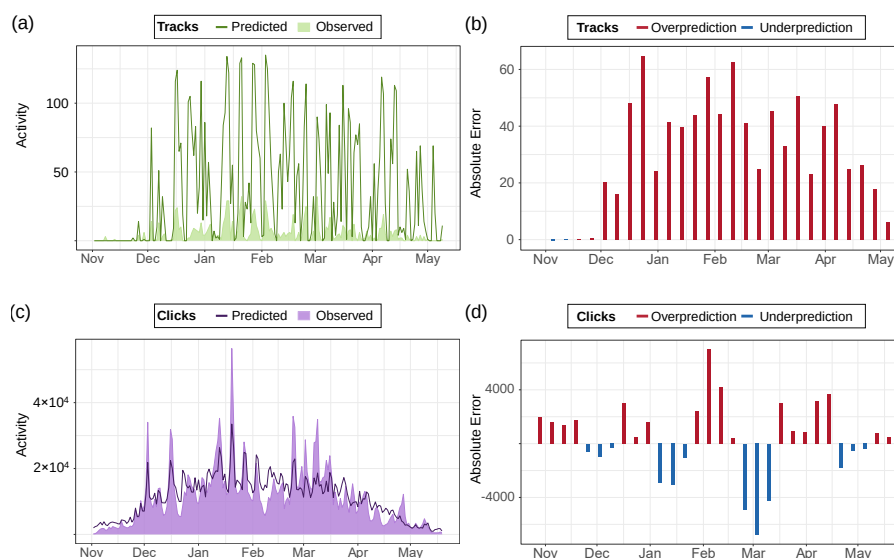
Figure 8. Temporal distribution of predictions and prediction errors for the example season 2023/24. Observed daily activity vs. predicted daily activity obtained from (a) the track model and (c) the click model. Counts were aggregated over the whole study area. Absolute prediction delta from (b) the track model and (d) the click model. The prediction delta was calculated as (b) the weekly mean absolute difference between number of regions where activity was predicted and number of regions where activity was observed and (d) the weekly mean absolute difference between predicted and observed clicks.
