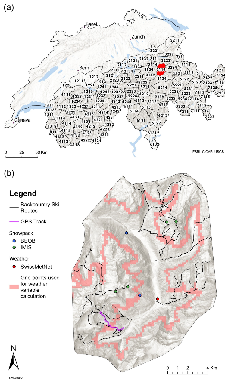
Figure 2. (a) Map of Switzerland showing 128 Alpine warning regions, the smallest spatial units used to communicate avalanche danger in the avalanche forecasts in Switzerland. Each region is labelled with its respective warning region code (WRC). (b) Example region 3113, highlighted in (a), showing weather stations (SwissMetNet), snow measurement stations from automatic measuring stations (IMIS) and from manual measuring stations (BEOB), backcountry ski routes featured on www.skitouren.guru.ch , one example GPS track, and the elevation belt used to calculate meteorological variables by averaging all grid points that lie within. To obfuscate exact GPS locations, each GPS track has only the warning region code (3113 in this example) as spatial reference.
