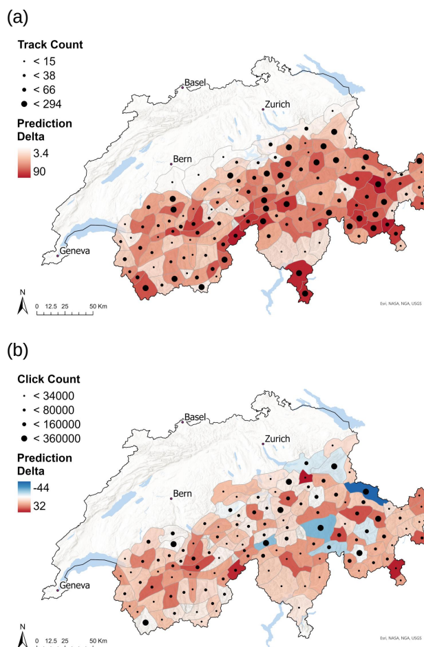
Figure 7. Mean prediction error for (a) track model and (b) click model across all seasons, where red indicates that the model overpredicted and blue indicates that the model underpredicted activity. (a) The prediction error was calculated as (a) the mean number of days per season with a false positive prediction and (b) the mean daily difference between predicted and observed clicks. Black circles indicate the total number of tracks (a) or clicks (b) per region.
