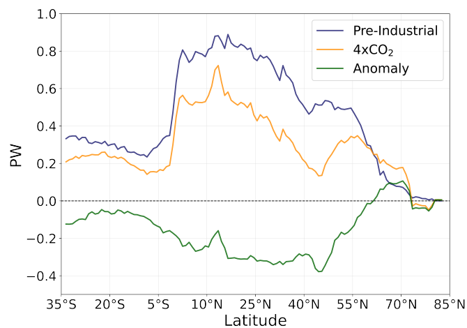
Figure 5. Atlantic Ocean meridional heat transport for PI and 4xCO_2 .
