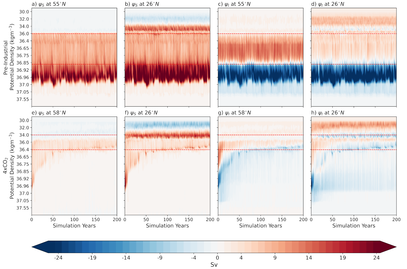
Figure 6. Hovmöller diagrams of surface and interior transformations in density space for PI (upper panels) and 4xCO 2 (bottom panels). First two columns (a, b, e, f) display the surface transformations, \psi_S , at (a, e) the \rho -AMOC maximum latitude and (b, f) 26°N, while last two columns (c, d, g, h) display the interior transformations, \psi_I , at (c, g) the \rho -AMOC maximum latitude and (d, h) 26°N. Positive (red) values indicate transformations toward lighter waters (buoyancy gain/upwelling), and negative (blue) values indicate transformations toward denser waters (buoyancy loss/downwelling). Red dashed lines denote the upper and lower density bounds of the \rho -AMOC upper limb, computed from the mean over the last 50 years of each simulation. The \rho -AMOC maximum latitude for both simulations is displayed in Table 22.1.
