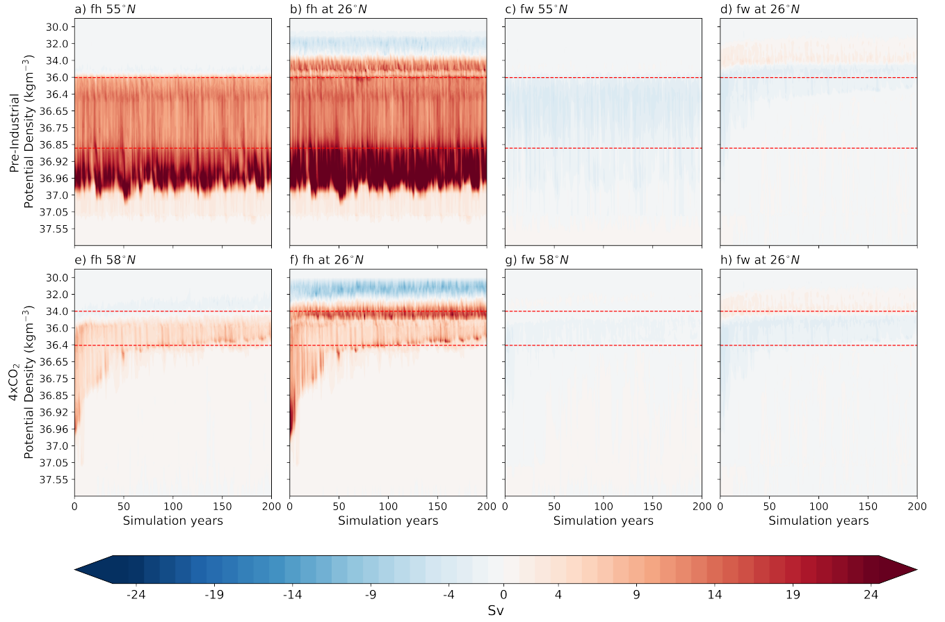
Figure A1. Hovmöller diagrams of the contributions of heat fluxes (FH) and freshwater fluxes (FW) to surface transformations for PI (upper panels) and 4xCO 2 (bottom panels). First two columns (a, b, e, f) display the FH at (a, e) the \rho -AMOC maximum latitude and (b, f) 26°N, while last two columns (c, d, g, h) display the FW at (c, g) the \rho -AMOC maximum latitude and (d, h) 26°N. Positive (red) values indicate transformations toward lighter waters (buoyancy gain/upwelling), and negative (blue) values indicate transformations toward denser waters (buoyancy loss/downwelling). Red dashed lines denote the upper and lower density bounds of the \rho -AMOC upper limb, computed from the mean over the last 50 years of each simulation. The \rho -AMOC maximum latitude for both simulations is displayed in Table ?? .
