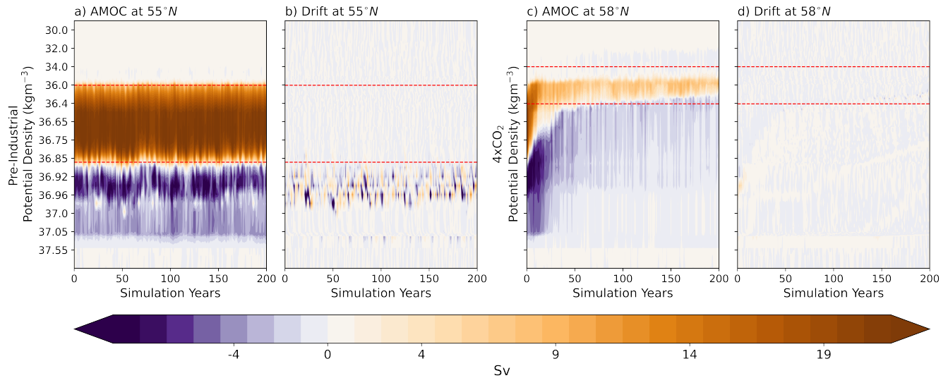
Figure A2. Hovmöller diagrams of \rho -AMOC (a,c) and model drift (b,d) in density space for PI (a,b) and 4xCO 2 (c,d). Red dashed lines denote the upper and lower density bounds of the \rho -AMOC upper limb, computed from the mean over the last 50 years of each simulation. The \rho -AMOC maximum latitude for both simulations is displayed in Table 1.
