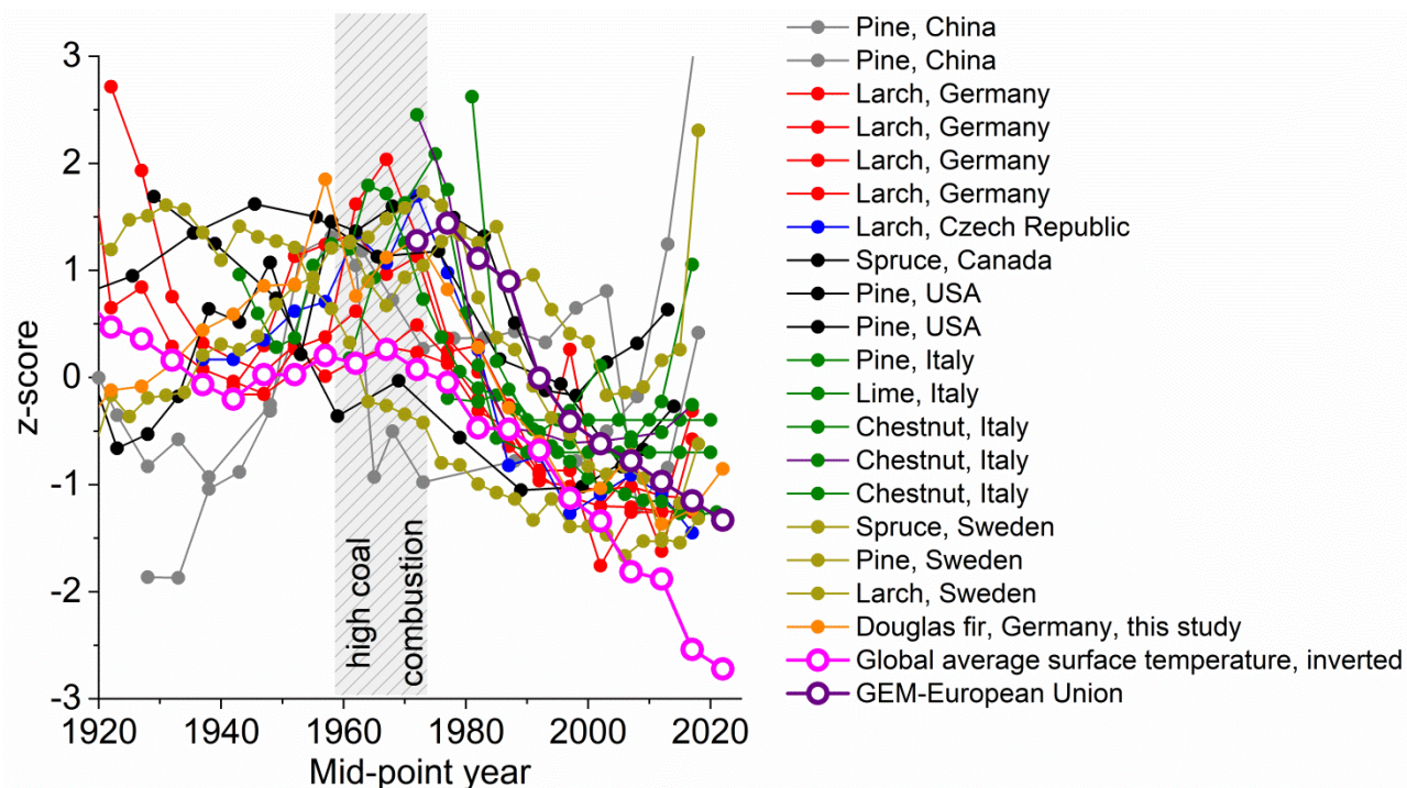
Fig. 4: Records of tree-ring mercury concentration (filled points) at different sites in the Northern Hemisphere (colors refer to countries) Scanlon et al., 2020; Chellman et al., 2020; Ghotra et al., 2020; Nováková et al., 2021; Wang et al., 2021; Baroni et al., 2023; Peng et al., 2024; Fornasaro et al., 2023 and records (circles) of global average surface temperature (inverted) and atmospheric mercury concentration emitted in the European Union. The grey shaded area shows the period of intense coal combustion in Europe according to Streets et al. (2019).
