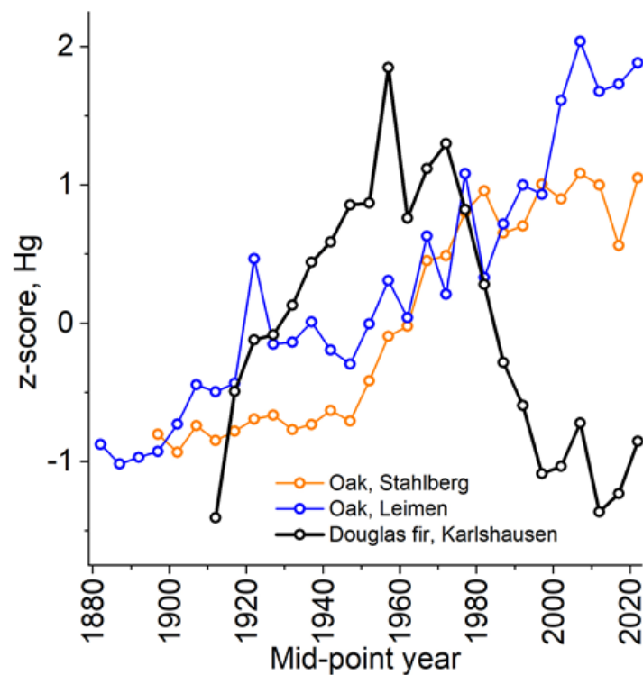
220 Fig. 3: Tree-ring mercury (Hg) records at the investigated oak (Stahlberg, Leimen) and Douglas fir (Karlshausen) sites in Rhineland-Palatinate, Germany.
