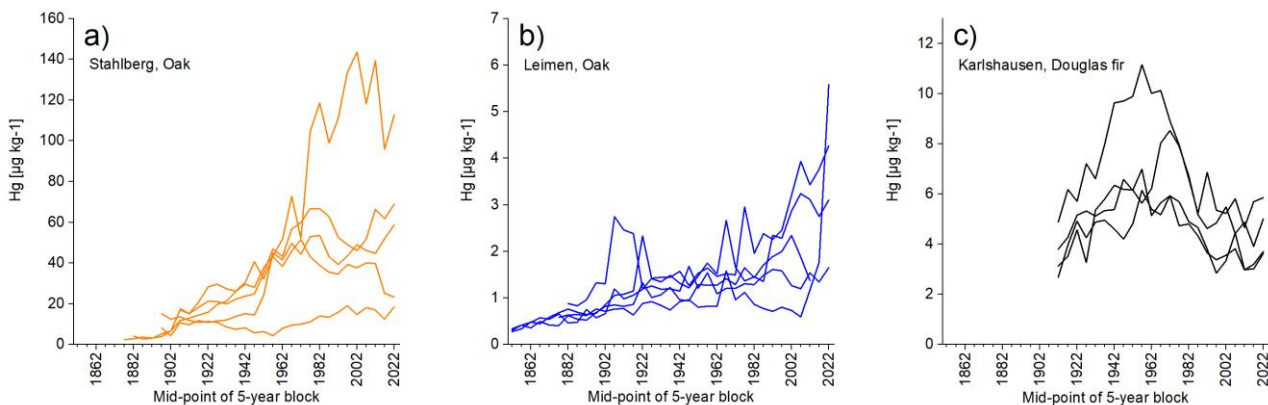
Fig. 2: Tree-ring mercury (Hg) concentration in individual trees through time from three locations in Rhineland-Palatinate, Germany.
