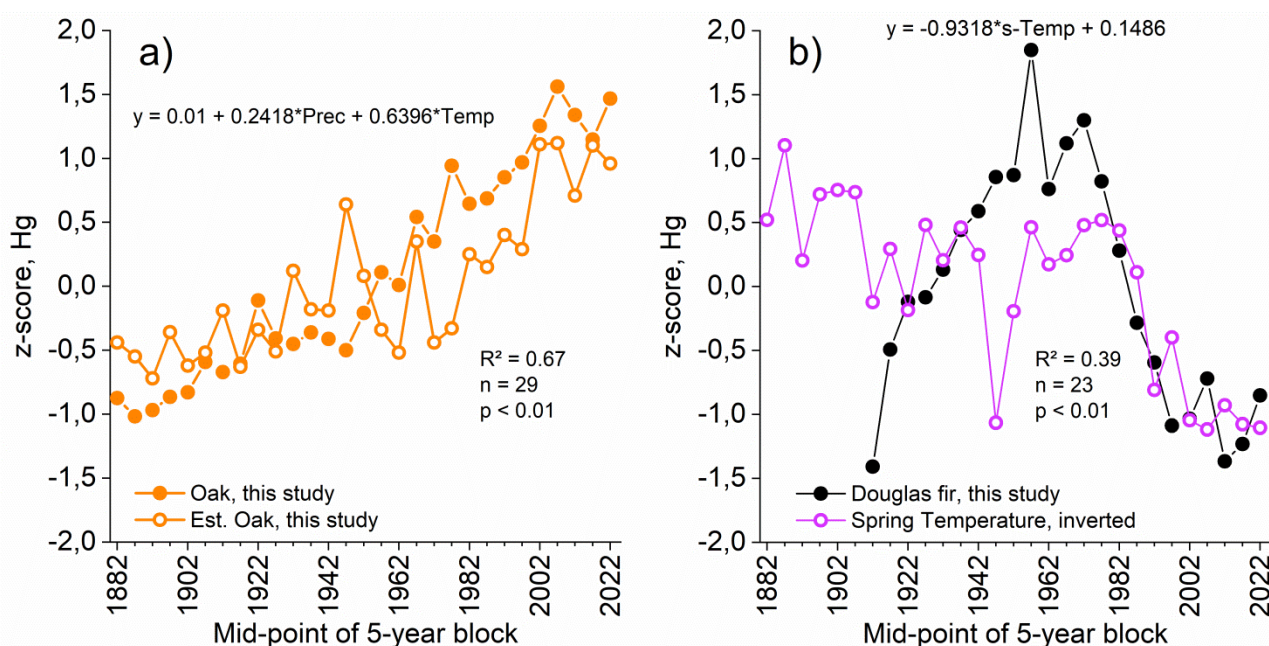
345 Fig. 5: Climate response of tree-ring mercury (Hg) concentration variability for oak (a) and Douglas fir (b). Tree-ring Hg concentration in oak trees can be estimated by spring-summer mean air temperature (Temp) and spring-summer precipitation sum (Prec) and by spring mean air temperature (s-Temp) for Douglas fir trees (b).
