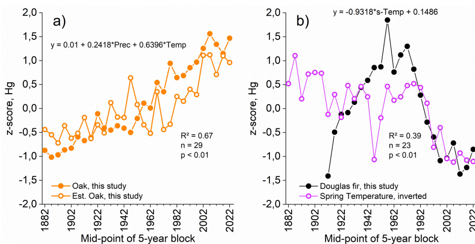
Figure 5: Climate response of tree-ring mercury (Hg) concentration variability for oak (a) and Douglas fir (b). Tree-ring Hg concentration in oak trees can be estimated by spring-summer mean air temperature (Temp) and spring-summer precipitation sum (Prec) and by spring mean air temperature (s-Temp) for Douglas fir trees (b).
