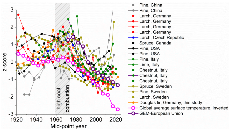
Figure 4: Records of tree-ring mercury concentration (filled points) at different sites in the Northern Hemisphere (colors refer to countries) Scanlon et al., 2020; Chellman et al., 2020; Ghotra et al., 2020; Nováková et al., 2021; Wang et al., 2021; Baroni et al., 2023; Peng et al., 2024; Fornasaro et al., 2023 and records (circles) of global average surface temperature (inverted) and atmospheric mercury concentration emitted in the European Union. The grey shaded area shows the period of intense coal combustion in Europe according to Streets et al. (2019).
