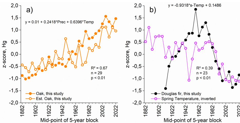
Fig. 5: Climate response of tree-ring mercury (Hg) concentration variability for oak (a) and Douglas fir (b). Tree-ring Hg concentration in oak trees can be estimated by spring-summer mean air temperature (Temp) and spring-summer precipitation sum (Prec) and by spring mean air temperature (s-Temp) for Douglas fir trees (b).
