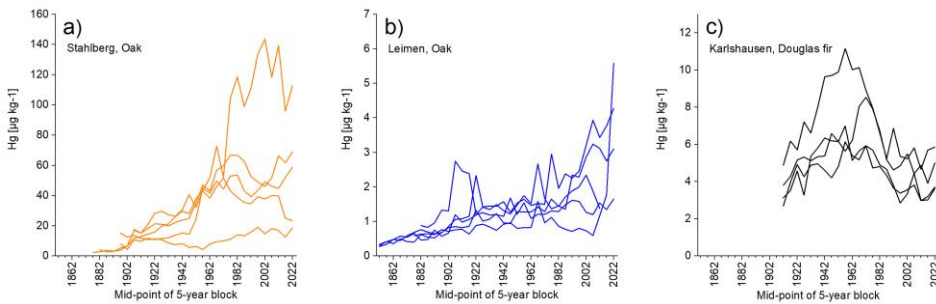
Fig. 2: Tree-ring mercury (Hg) concentration in individual trees through time from three locations in Rhineland-Palatinate, Germany.
