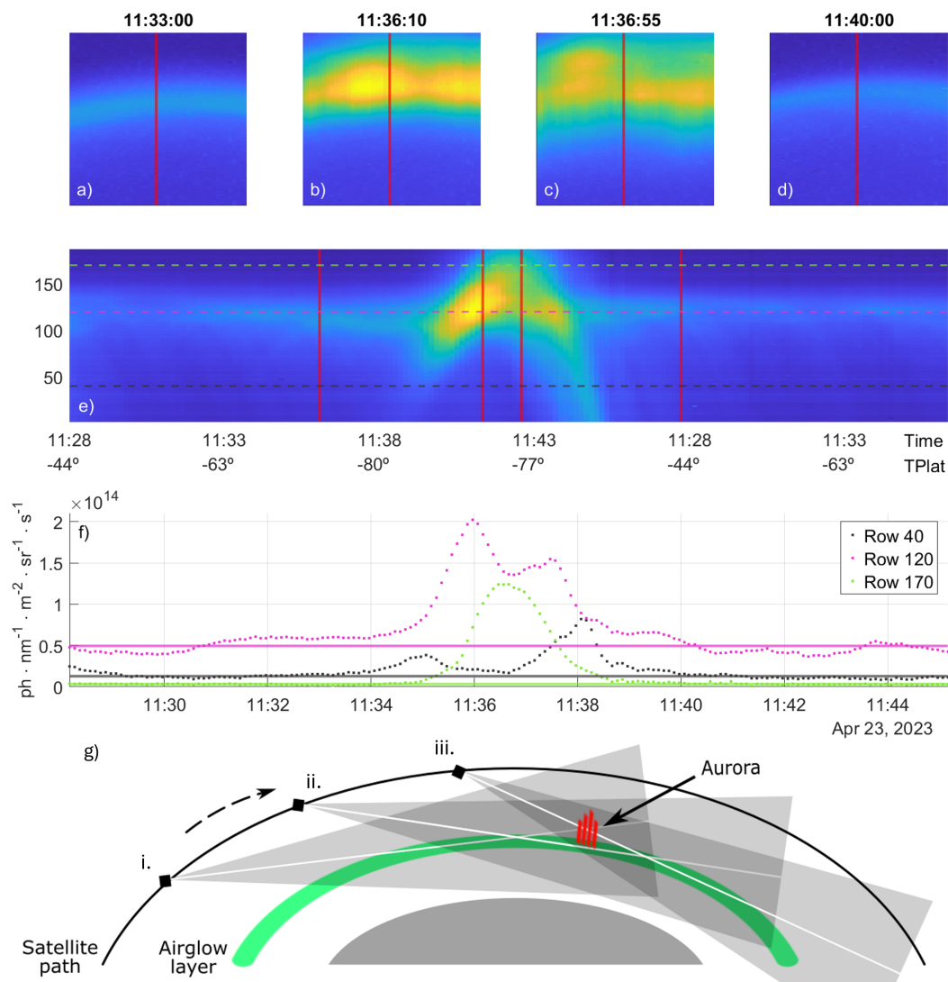
Figure 1. a-d) Processed images taken by the limb instrument at the times indicated on top of each panel. e) Keogram created by adding the central column of each image in chronological order. Vertical red lines indicate the columns corresponding to the images in panels a-d). Horizontal lines correspond to the rows plotted in the next panel. f) Pixel values of three rows of the keogram (dots) together with the fitted background (solid line). g) 2D sketch of MATS perspective of aurora (not to scale), corresponding to the peak of the parabola in the keogram (ii.), and when observed below the airglow before the peak (i.), and after (ii.). The grey area represents the instrument's field of view, while the white line is the tangent line.
