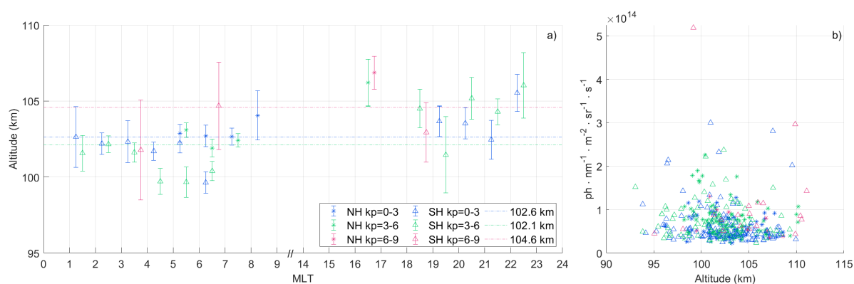
Figure 3. a) One-hour average of auroral event altitudes as a function of MLT. Asterisks represent the northern hemisphere, while triangles represent the southern hemisphere. Blue includes events with Kp-index between 0 and 3, green between 3 and 6, and red between 6 and 9. Error bars indicate the standard error of the mean. Horizontal dashed lines indicate the averaged altitude of all events in each of the Kp-index bins. b) Intensity as a function of altitude for all events analyzed. Colors and markers follow the same pattern as in a).
