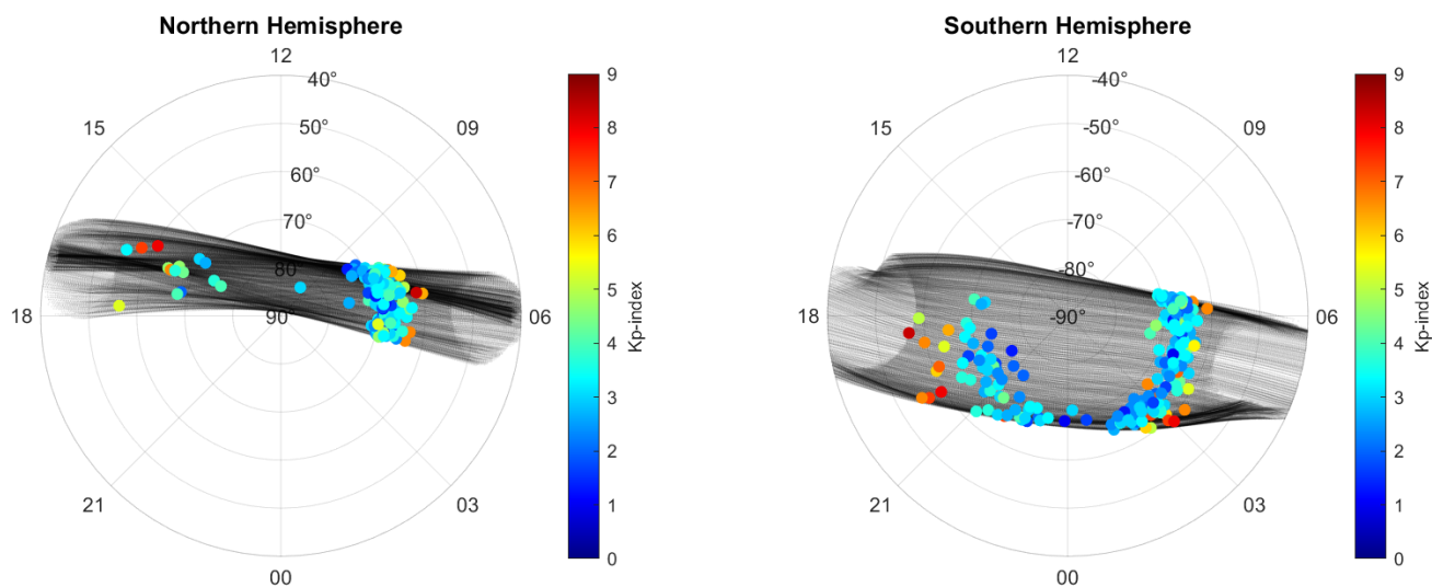
Figure 2. Distribution of the analyzed events in MLT plots for the northern hemisphere (left) and southern hemisphere (right). Color indicates the Kp-index of each event.
