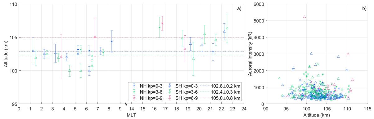
Figure 3. a) Average altitude of events occurring within the same one-hour bin as a function of MLT. Asterisks represent the northern hemisphere, while triangles represent the southern hemisphere. Blue includes events with Kp-index between 0 and 3, green between 3+ and 6, and red between 6+ and 9. Error bars indicate the standard error of the mean. Horizontal dashed lines indicate the averaged altitude of all events in each of the Kp-index bins. The mean values are indicated in the legend together with the uncertainty of the mean. b) Intensity as a function of altitude for all events analyzed. Colors and markers follow the same pattern as in a).
