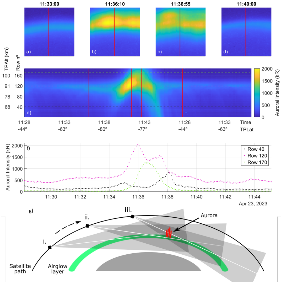
Figure 1. a-d) Processed images taken by the limb instrument at the times indicated on top of each panel. The colormap limits are the same as in panel e). e) Keogram created by adding the central column of each image in chronological order. X-axes indicate time and latitude of the tangent point (TPLat). Y-axes represent the row number and the average (among all times) altitude of the tangent point corresponding to each pixel row (TPAlt). Vertical red lines indicate the columns corresponding to the images in panels a)-d). Horizontal lines correspond to the rows plotted in the next panel. f) Pixel values of three rows of the keogram (dots) together with the fitted background (solid line). g) 2D sketch of MATS perspective of aurora (not to scale), corresponding to the peak of the parabola in the keogram (ii.), and when observed below the airglow before the peak (i.), and after (iii.). The grey area represents the instrument's field of view, while the white line is the tangent line.
