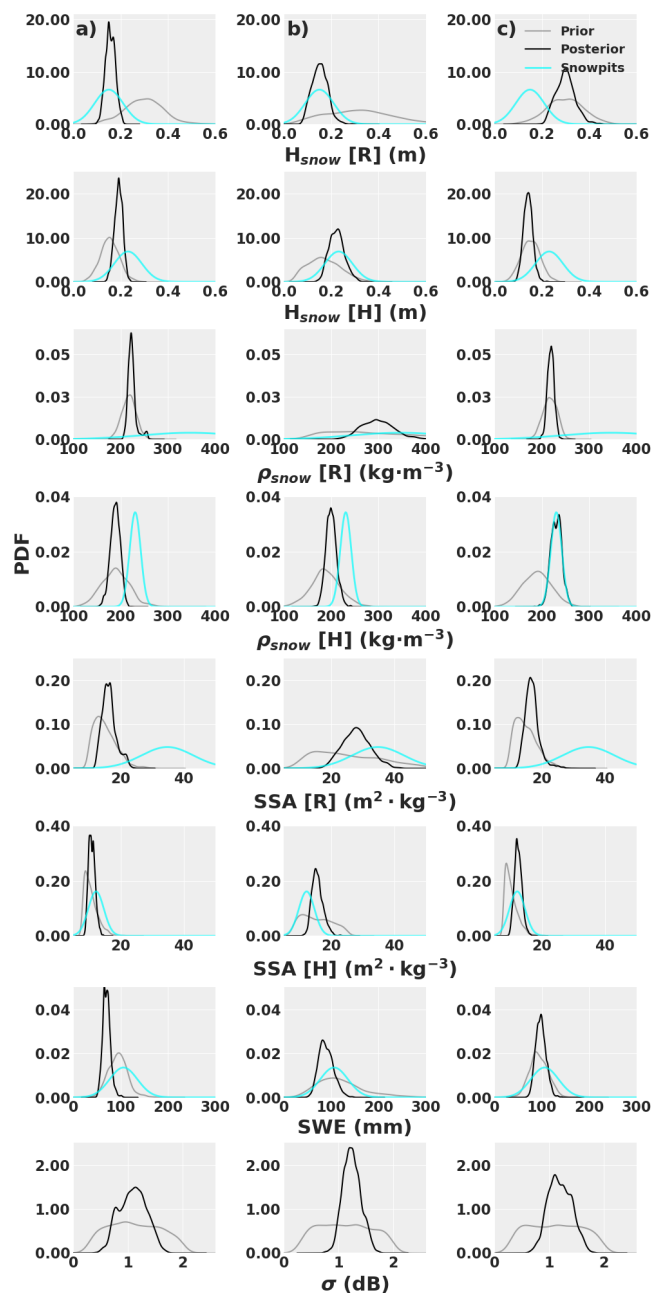
Figure 10. Example from the SM site of prior distributions coming from the default (column a) and Arctic (column b) versions of SVS-2 and retrieved posterior distributions from the MCMC method, for the different snow variables compared to the surveyed snow measurements. Column c) consists in the MCMC optimization using the default version of SVS-2, where no vertical constraints on snow properties were applied. \sigma is the free parameter corresponding to the uncertainty of the radar backscatter measurement and was not measured in the field.
