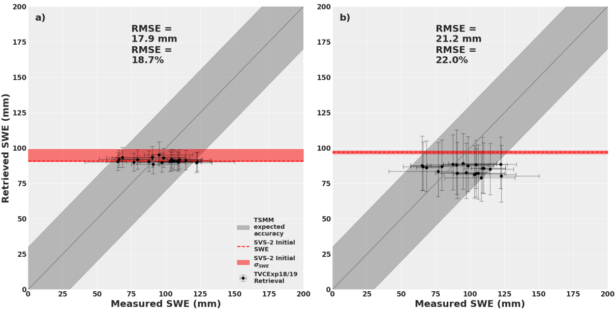
Figure 8. Comparison of the retrieved SWE using the MCMC approach with priors coming from the top 30 ensemble members of the default and Arctic versions of SVS-2 (Woolley et al., 2024). The error bars show the 1st and 3rd quartiles of the measured (x-axis) and posterior (y-axis) distributions.
