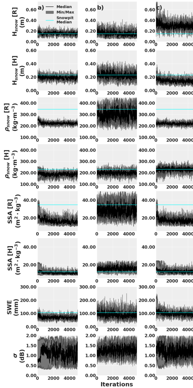
Figure 11. Evolution of the MCMC sampling for the 5000 iterations which correspond to the posterior distributions of Figure 10 for the same three optimization scenarios. Horizontal lines consist in median values from measurements (snowpits).
