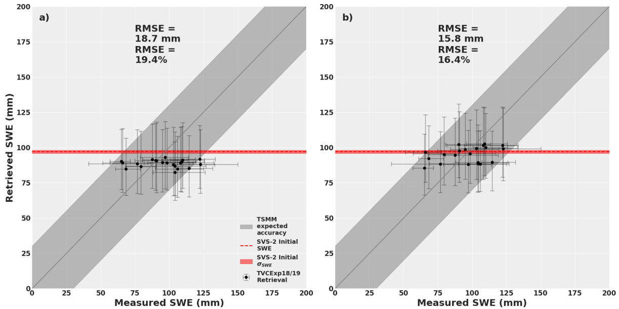
Figure 9. Comparison of the retrieved SWE using the MCMC approach with priors coming from the top 30 ensemble members of the Arctic versions of SVS-2 (Woolley et al., 2024) and a higher prior uncertainty on the SSA ( \sigma_{SSA} ) and an adding three more observations (different incidence angles), emulating the number of observations the TSM would acquire. The error bars show the 1st and 3rd quartiles of the measured (x-axis) and posterior (y-axis) distributions.
