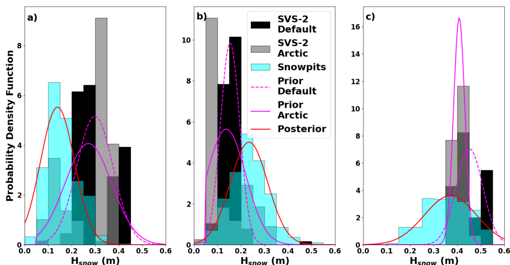
Figure 3. Measured snow thickness ( H_{\text{snow}} ) distributions during the January TVC campaign, compared to the thickness distributions provided but the 120 SVS-2 ensemble members (Woolley et al., 2024) for the two dominant snow grain type layers a) rounded grains, b) depth hoar, and c) the total thickness, including both snow layers. Magenta lines represent the truncated normal distributions (Table 1) used as priors, using the mean and standard deviations of the two different SVS-2 versions. The red line represents the normal distribution, using the mean and standard deviation of the measurements, and consists in the desired posterior distributions obtained by the MCMC approach.
