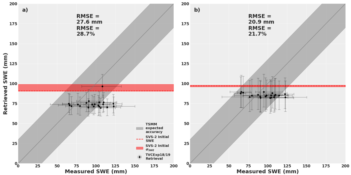
Figure 7. Comparison of the retrieved SWE using the MCMC approach with priors coming from all 120 ensemble members of the a) default and b) Arctic versions of SVS-2 (Woolley et al., 2024). The error bars show the 1st and 3rd quartiles of the measured (x-axis) and posterior (y-axis) distributions.
