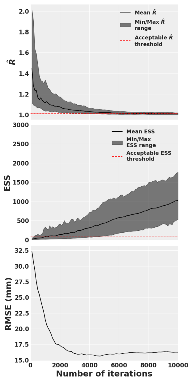
Figure 6. Evolution of a) \hat{R} (Gelman and Rubin, 1992), b) Equivalent Sample Size (ESS) (Martin et al., 2021) for all variables, all sites, and seven chains; and the SWE RMSE over the 10,000 iterations of the MCMC optimization. Acceptable \hat{R} threshold published by Vehtari et al. (2021), and ESS threshold published by Kass et al. (1998) are shown in red.
