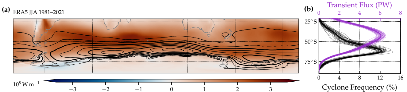
Figure 1. Climatologies of transient MSE fluxes and cyclone frequencies during SH winter (JJA). (a) Vertically integrated and seasonally averaged transient MSE fluxes, \langle v'm'_{MA} \rangle , (shading) are shown along with the cyclone mask frequency (black contours in steps of 5% starting at 5% with 15% and 30% highlighted in thicker contours). (b) Zonally integrated transient MSE fluxes, \langle [v'm'_{MA}] \rangle , (purple) and zonal mean cyclone frequencies (black) for individual seasons (thin lines) and the climatology thereof (solid lines). MSE fluxes are shown positive poleward. Note that the cyclone frequency in (b) is multiplied with the cosine of latitude for consistency.
