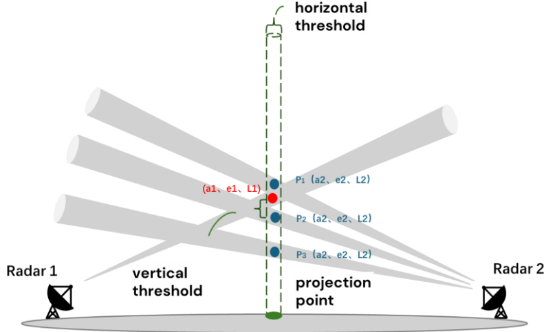
Figure 5. Schematic of two radars' spatial consistency algorithm.
