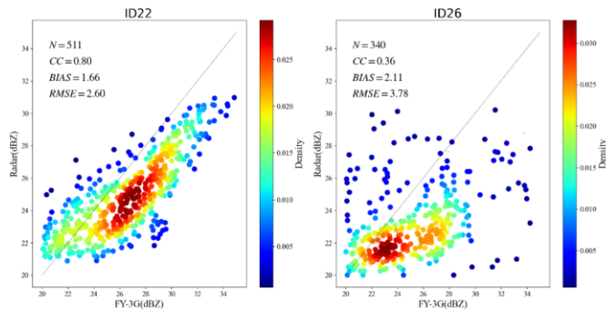
Figure 22. SGRCSatellite-ground consistency bias analysis results for individual X-band phased-array weather radars.
