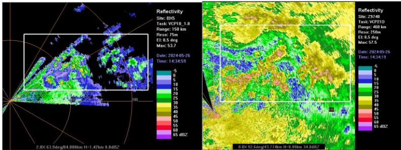
Figure 9. Comparison of reflectivity factors observed by adjacent X-band (left) and S-band (right) weather radars during a precipitation event on May 26, 2024, at 14:35.
