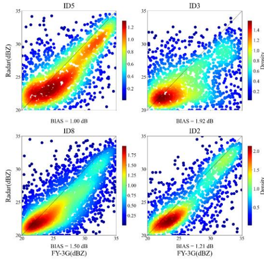
Figure 18. SGRCM Satellite-ground consistency analysis results for individual S-band weather radar stations.
