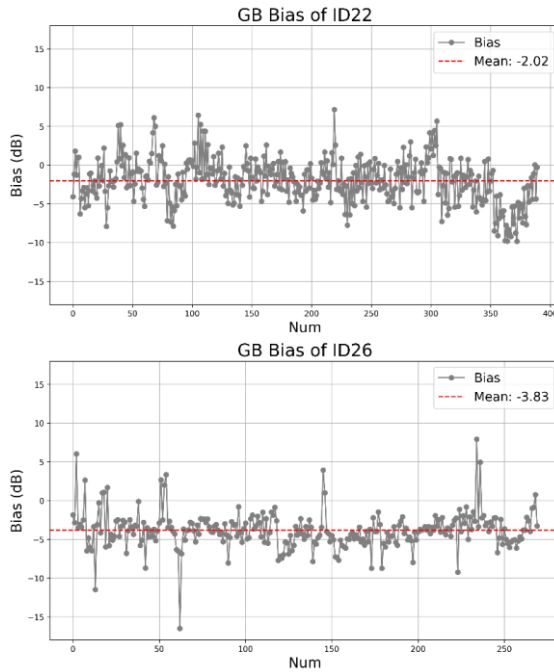
415 Figure 21. AWRCMground-based consistency bias analysis results for individual X-band phased-array weather radars. Figure 22 shows the SGRCMsatellite-ground consistency analysis results for the two radars. The bias in the figure represents the reflectivity factor of the phased-array radar minus that of FY-3G, with values of 1.66 dB and 2.11 dB, respectively. This also indicates that the reflectivity factor observed by the X-band phased-array radars is weaker, but the bias results are smaller than the AWRCMground-based analysis results. The SGRCMsatellite-ground standard deviation of radar 004-ID22 is smaller than that of radar +60-ID26. From the bias distribution of overlapping observation points, it can be seen that the SGRCMsatellite-ground bias of radar +60-ID26 exhibits greater dispersion. A preliminary analysis indicates that the valid SGRCM comparison results for radar ID22 are mainly concentrated in August 2024, whereas those for radar ID26 span June–September. Owing to the longer time window, the precipitation types encountered are more diverse, which may lead to differences in the SGRCM scatter distributions. This conclusion, however, requires further verification and analysis with additional observational data.
