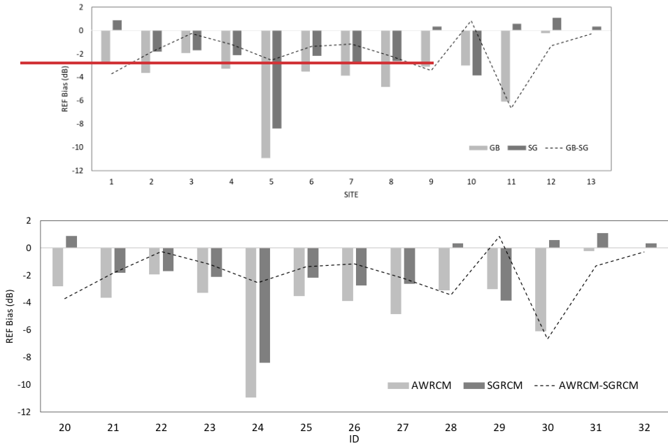
Figure 19. Comparison of mean bias between AWRCM and SGRCM ground-based and satellite-ground consistency for X-band phased-array weather radars in the South China region.
