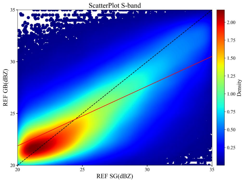
Figure 25. Scatter distribution of SGRCM satellite-ground-consistency results for S-band weather radars in China.
