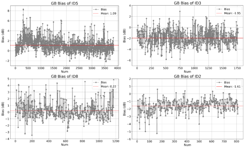
Figure 17. Bias analysis results of AWRCMground-based-consistency for individual S-band weather radar stations.
