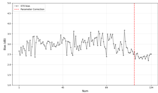
Figure 23. AWRCM Ground-based consistency results of the SC method radar in Sanya City, Hainan Province, before and after rectification. The gray line in the chart represents the variation in deviation, while the red dashed line indicates the rectification time.
