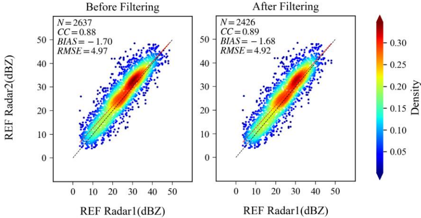
Figure 14. Consistency analysis results of the Guangdong Shantou radar with a adjacentnearby S-band weather radar before and after electromagnetic interference quality control. (Radar1 is the ID5, and Radar2 is ID8)
