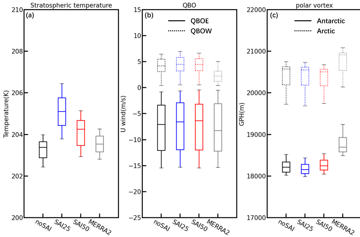
Figure S1: Box plots comparing stratospheric variability between model simulations and MERRA2 reanalysis (2000-2020). (a) near-global (60°S-60°N) temperatures at 100 mb; (b) QBO strength (tropical zonal mean zonal wind at 50 mb); (c) Antarctic polar vortex strength (denoted by the geopotential height averaged over 65°S-90°S at 50 mb) in the model and MERRA2 reanalysis dataset between year 2000 and 2020. Box plots show the median (horizontal line), 25th-75th percentiles (box), and 5 th -95 th percentiles (whiskers).
