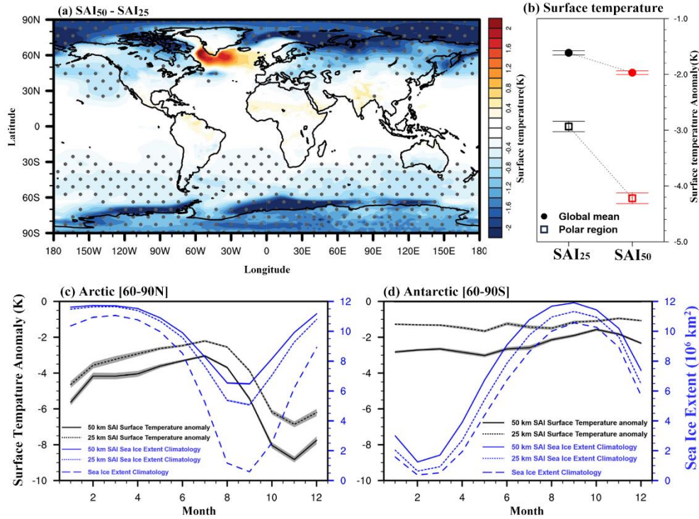
470 Figure 3: Less stratospheric warming and more polar surface cooling in the 50-km injection scenario (SAI 50 ) relative to the 25-km injection scenario (SAI 25 ). (a) The difference in the simulated annual mean surface temperature response between SAI 50 and SAI 25 . The stipple points denote the statistical significance at 95% level; (b) the simulated multi-annual and global mean temperature anomalies from SAI 25 and SAI 50 are denoted by the black and red filled dots, respectively. The temperature anomalies averaged in the polar regions are denoted in open squares. The error bars denote one standard deviation of the mean; (c) Simulated seasonal 475 distributions of the surface temperature anomalies in Arctic (60-90°N) due to SAI 25 and SAI 50 are shown in the solid and dashed red lines, respectively (left Y-axis). The error bars denote simulated standard deviation of the mean from ensemble simulations. The simulated seasonal variance of sea ice extent in Arctic (60-90°N) from the control (i.e. no SAI), SAI 25 , SAI 50 scenarios are denoted by the solid black, dashed blue and solid blue lines, respectively (right Y-axis); (d) same as (c) but for Antarctic (60-90°S).
