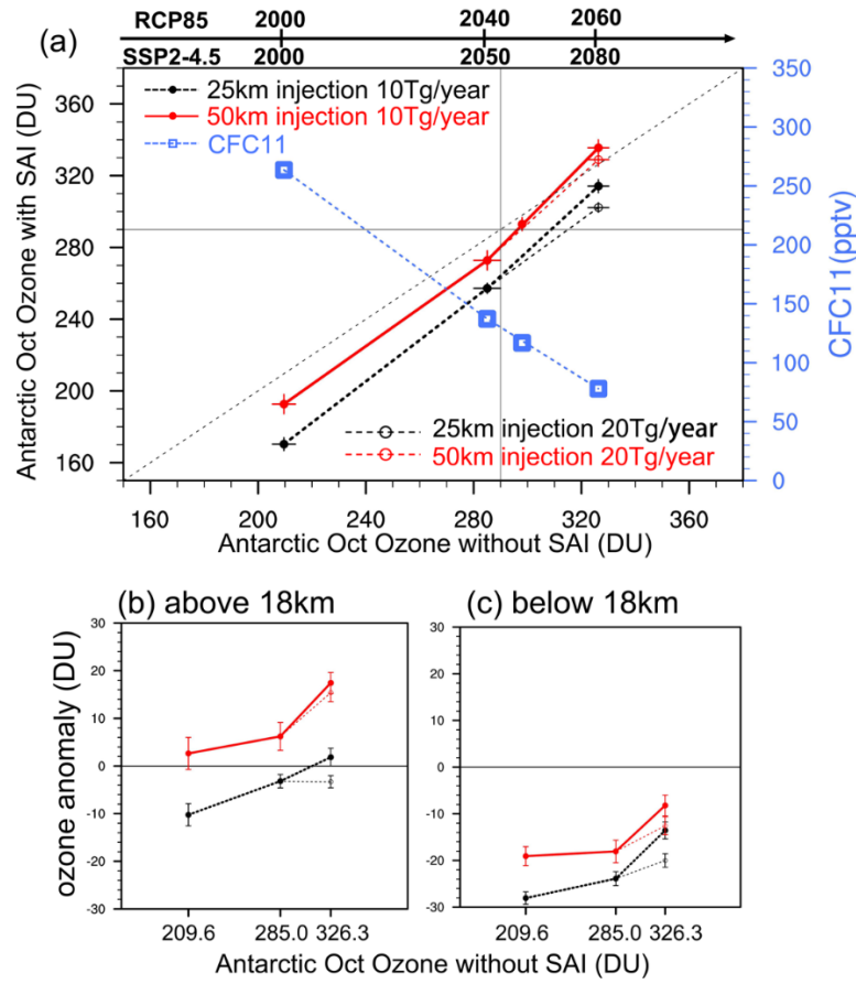
480 Figure 4: Reduced Antarctic ozone depletion in the 50-km injection scenario (SAI 50 ) relative to the 25-km injection scenario (SAI 25 ). (a) Snapshot simulations of the October Antarctic (60°S-90°S) total column ozone (TCO) averaged over a period of 15 years with and without SAI when the global mean surface mixing ratios of CFC-11 are around 270, 135, 117 and 70 pptv, respectively. For each CFC-11 mixing ratio, a total amount of 10 Tg per year of SO 2 is injected into two model grid boxes at 15°S and 15°N, respectively. In addition, SAI with 20 Tg SO 2 injected per year is simulated when the CFC-11 mixing ratio is around 70 pptv. TCO with 25-km (50-km) SAI with 10 Tg per year injection is denoted by the black (red) filled circles. TCO with 20 Tg per year injection is denoted by the open circles instead. The error bars denote the standard deviation of the mean from the ensemble simulations with details in Materials and Methods. The global mean surface CFC-11 mixing ratios are denoted by the blue squares (right axis). The estimated timeline of TCO from the RCP8.5 (Tilmes et al., 2020) and SSP2-4.5 (Macmartin et al., 2022) scenarios without SAI are denoted in the upper part of the panel. The black dashed line denotes equal TCO between simulations with and without SAI. The TCO value in 1980 (i.e. ~290 DU) is denoted by the thin black line; (b) simulated October Antarctic column ozone anomalies above 18 km with variant mixing ratios of CFC-11. The simulated TCO anomalies with SAI injections (10 Tg per year) at 25-km and 50-km are denoted by the black and red filled circles, respectively. TCO anomalies with the injection rate of 20 Tg per year are denoted by the open circles. The error bars denote the simulated 1 \sigma uncertainty from the ensemble simulations; (c) same as (b) but for the column ozone anomalies from the ground to 18 km.
