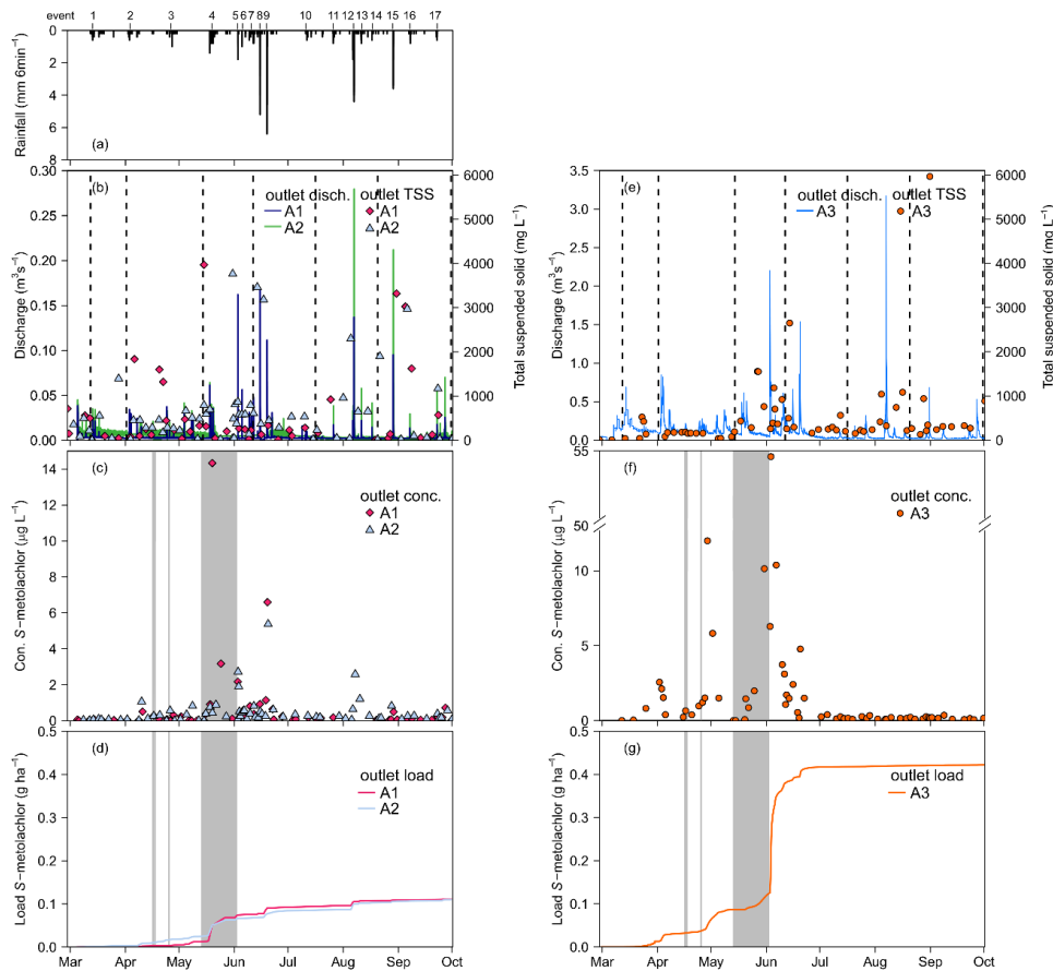
Figure 2: Dynamics of rainfall, river discharge, suspended solid and S-metolachlor concentration at the outlet of the sub-catchment A1, A2 (left panel) and Souffel catchment A3 (right panel) in 2019. (a) Rainfall at location R1 (Fig. 1), (b & e) River discharge at A1 & A2 and total suspended solids at A3, (c & f) S-metolachlor concentrations in dissolved phase ( n_{A1} = 58 ; n_{A2} = 68 ; n_{A3} = 176 ) and (d & g) Cumulative area-normalised load in dissolved phase. Dashed vertical line in (b & e) represents the timing of the seven grab sampling campaigns. The shaded gray area in (c, d, f, g) indicates the dates of S-metolachlor application.
