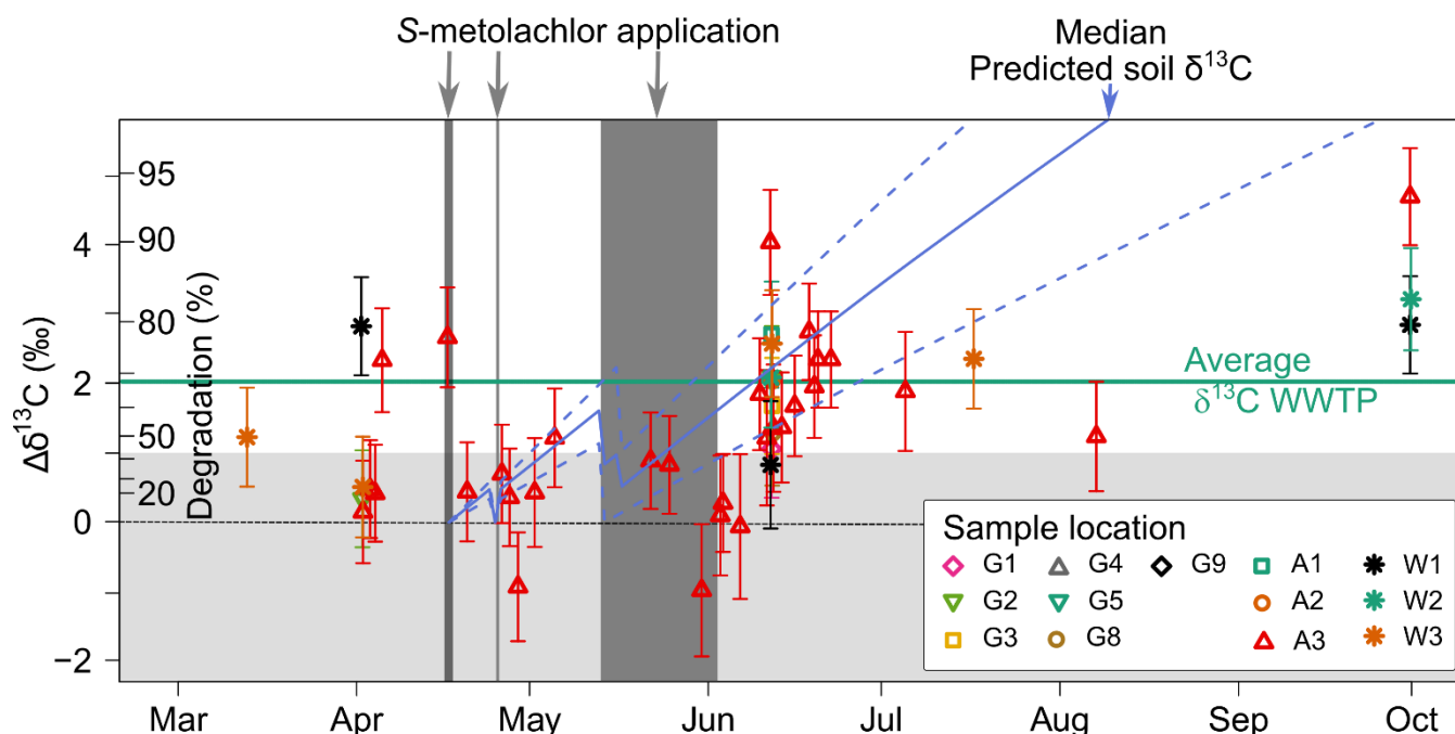
Figure 4: Carbon stable isotope fractionation ( \Delta\delta^{13}C = \delta^{13}C(t) - \delta^{13}C_0 ) of S-metolachlor in river ( n=61 ) water across the growing season compared to the predicted topsoil \delta^{13}C values. The colored dashed lines indicate the median uncertainty in the topsoil \delta^{13}C values within \pm 0.5\% (see Table S7 in the Supplement). The shaded light grey area represents the minimal change in isotope signature ( \Delta\delta^{13}C_{min} , calculated as per Eq. S1 in the Supplement) in water, beyond which significant isotope fractionation can be attributed to degradation, thereby representing the threshold for detecting biodegradation. The dark grey segment denotes the estimated date of S-metolachlor application ascertained from the farmer survey within sub-catchment G11. The green line represents the average \delta^{13}C value from wastewater treatment plant data ( n=9 ). The black dash line represents the \Delta\delta^{13}C = 0\% value. Error bars encompass the propagation of uncertainty associated with \Delta\delta^{13}C .
