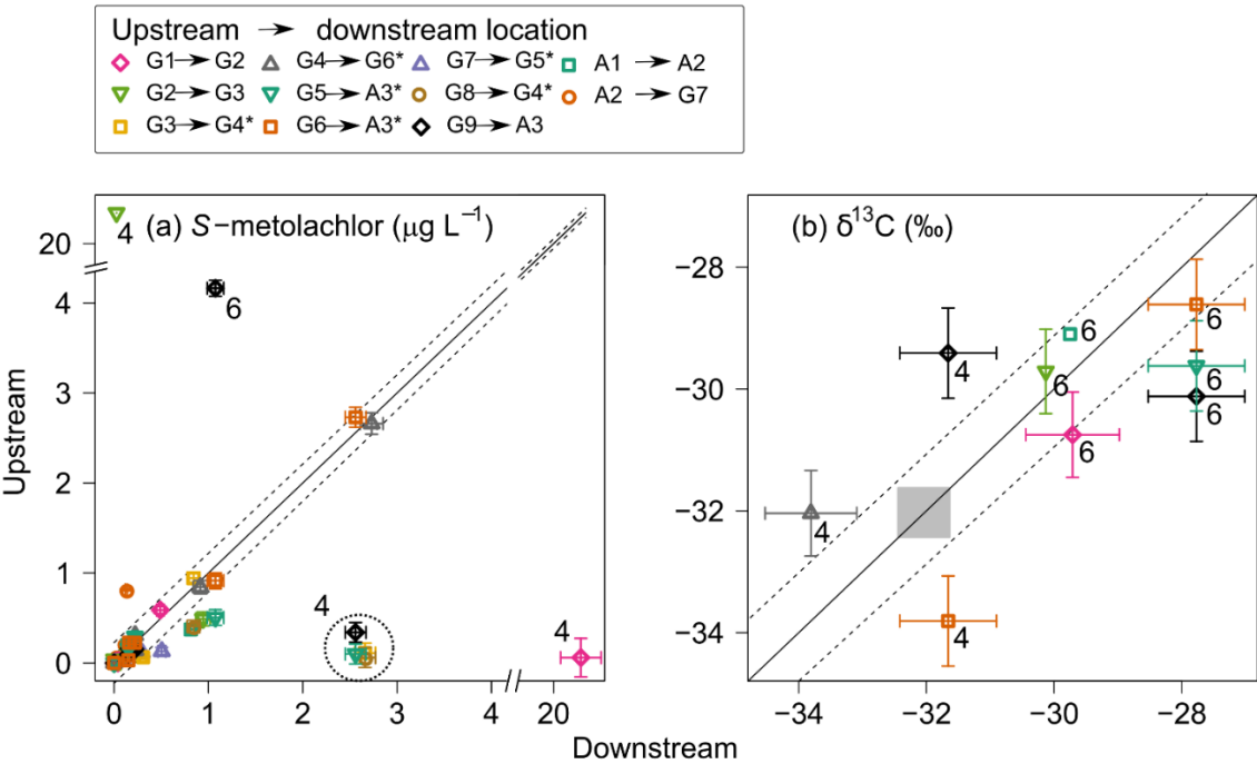
Figure 3: Dynamics of S -metolachlor from upstream to downstream for the river reaches. S -metolachlor (a) concentrations and (b) carbon stable isotope composition ( \delta^{13}\text{C} ) in April (label 4) and June (label 6). The black solid line illustrates a 1:1 relationship, whereas the dashed line signifies the 95% confidence interval associated with the measurements. The grey zone illustrates the initial isotope composition of S -metolachlor commercial formulation ( \delta^{13}\text{C}_0 = -31.8 \pm 0.3\text{‰} ). Error bars denote the propagation of uncertainty from triplicate measurements for both concentration and \delta^{13}\text{C} . Asterisks (*) denotes reaches receiving WWTP effluent.
