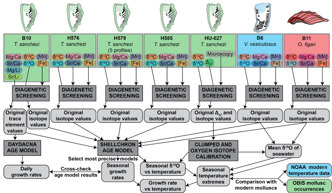
313 314 Figure 3: Flowchart of data processing steps carried out for this study.
