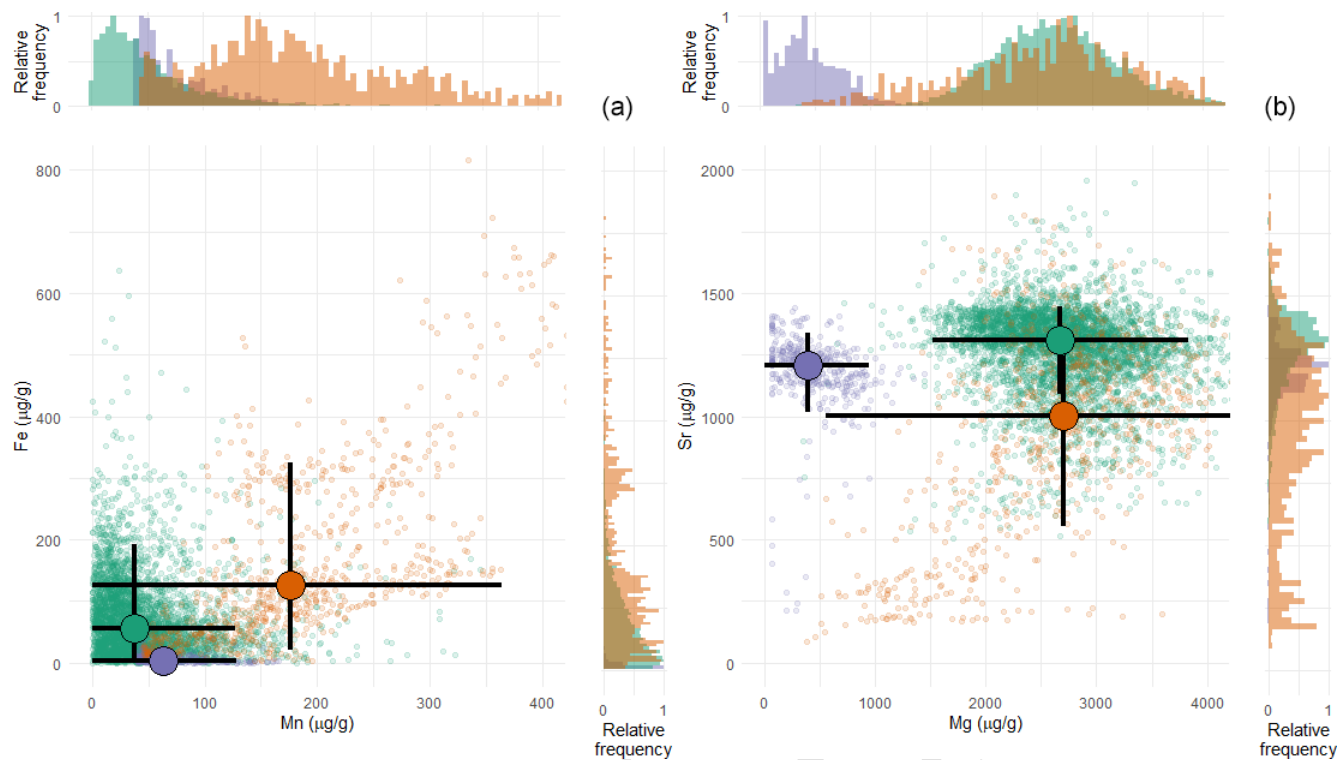
Figure 5. Cross plots of manganese vs. iron (a) and magnesium vs. strontium (b) concentrations in T. sanchezi (green), V. vesiculosus (purple) and O. figari (orange) measured using micro-XRF line scan analysis. Shaded points highlight individual measurements in profiles through the shells while bold black crossed lines highlight median concentration values with 2 standard deviations of the variability per species. Histograms on the edges of the plot show the distribution of concentration values in the dataset per element.
