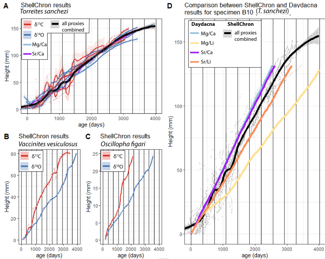
Figure 6. Plot of shell height vs. age in all specimens based on ShellChron modelling on Mg / Ca, Sr / Ca, \delta^{18}\text{O}_\text{c} and \delta^{13}\text{C} profiles in T. sanchezi (A), \delta^{18}\text{O}_\text{c} and \delta^{13}\text{C} profiles in V. vesiculosus (B) and \delta^{18}\text{O}_\text{c} and \delta^{13}\text{C} profiles in O. figari (C). Solid lines represent LOESS smoothed curves (span = 0.2) through the age-height data, with shaded areas indicating uncertainties around the growth models. (D) Comparison between ShellChron results for T. sanchezi specimen B10 profiles (combined chronology from all proxies; black line in panel (A)) and Daydacna results on subdaily-scale trace element profiles through the same specimen. Colours of curves and uncertainty envelopes represent the proxy on which age modelling was based (see legends in top-left corners of the panels).
