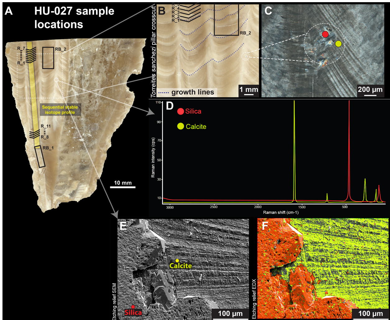
Figure 2. (A) High-resolution colour scan of a cross-section through T. sanchezi specimen HU-027 with the location of samples for \delta^{18}\text{O} , \delta^{13}\text{C} (yellow rectangle) and clumped isotope analysis (black text and lines). (B) Zoomed-in insert showing fine lamination in columns through HU-027, the location of samples RB_2 and R_1–R_5, and examples of isochronous growth lines (dashed lines) that link the timing of growth between pillars in the cross-section. (C) Cross-polarized light image of the edge of a shell column showing locations for characterizing diagenetic (silicified) and pristine areas in the shell. (D) Raman spectra of pristine calcite (yellow) and silicified (red) areas in the shell of HU-027. (E) Scanning Electron Microscopy for scatter image of the area of interest highlighted in B, showing original calcite shell structures (right) and silicified areas of the shell (left). (F) Energy-dispersive X-ray spectroscopy (EDS) image of the same area shown in panel (E) showing the silicon (red) and calcium (yellow) composition on a micrometre scale.
