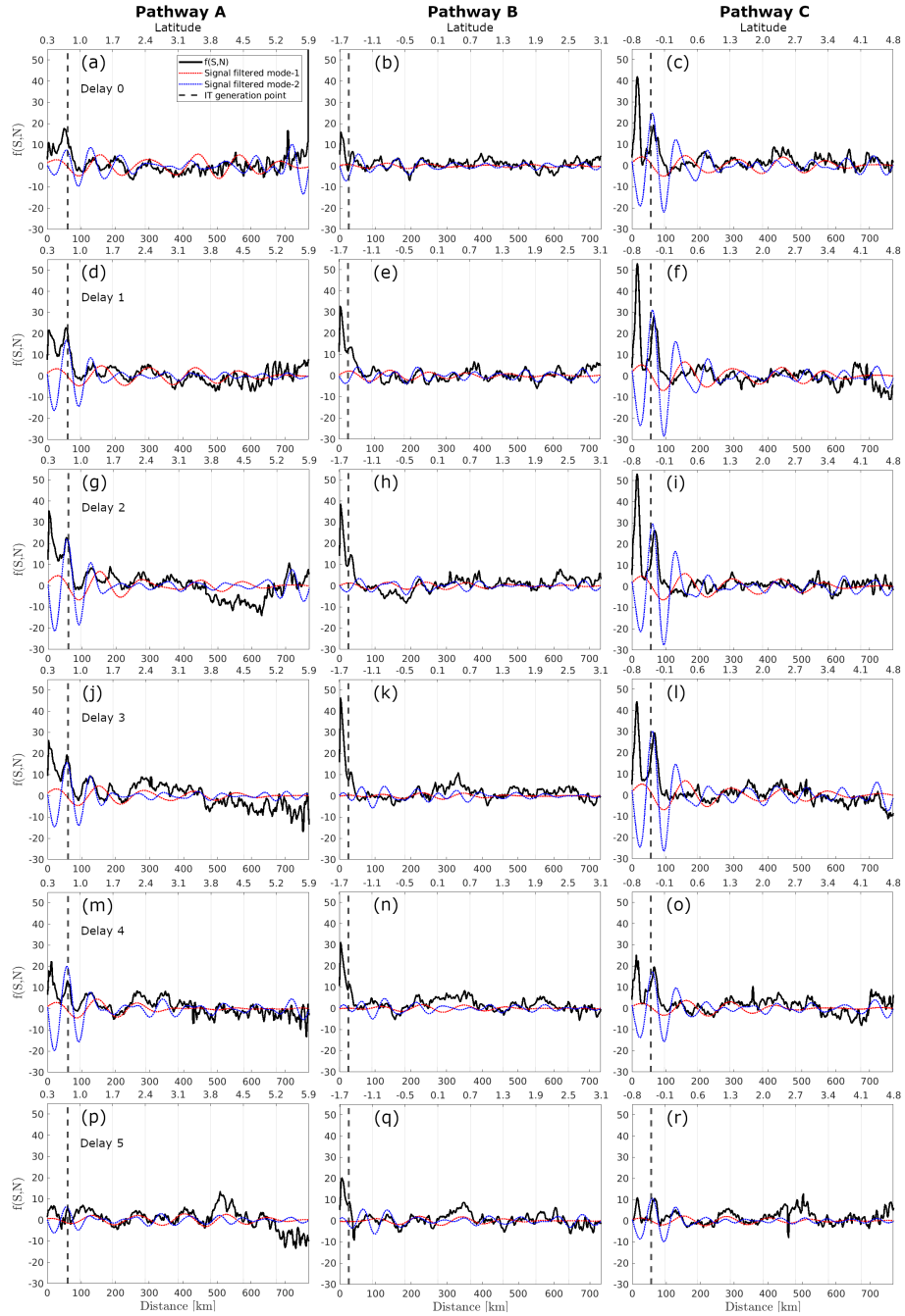
Figure 10. Profiles along the A, B, and C pathways (columns) of the spring-neap tidal cycle CHL composite using MODIS-Aqua, considering delays of 0-5 days. black and dashed red and blue lines represent, respectively, the original signal and the signal filtered for mode-1 (100-150 km) and mode-2 (50-100 km) wavelengths.
