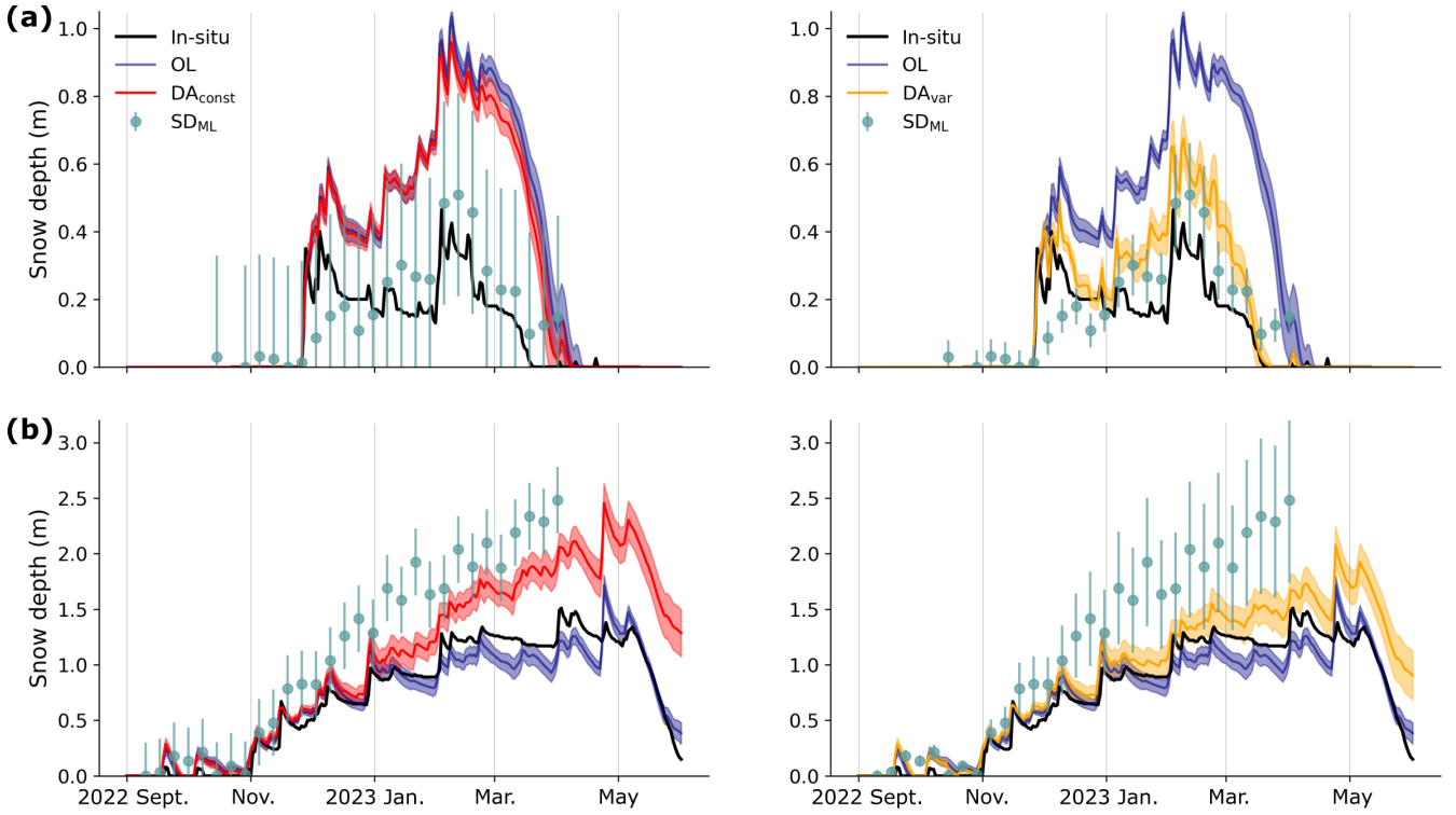
Figure 2. Snow depth estimates and independent in-situ measurements at two example sites. (a) Snow depth from DA const (red, left) and DA var (orange, right) compared with the OL (navy) from a measurement station in Austria ( \sim 13.6228^\circ E , 47.0944^\circ N , 1050 m elevation). The shading represents \pm 1 standard deviation in the model ensembles. The sage green dots represent the assimilated SD ML retrievals, with error bars for the assumed observation error standard deviation ( \sigma_{obs} , Equation 2). (b) Same as (a), but for a different measurement station in Switzerland ( \sim 7.7836^\circ E , 45.9872^\circ N , 2948 m elevation). These two sites were chosen due to a lack of gaps in the in-situ measurements and their general representativeness of locations where the DA removes and adds snow.
