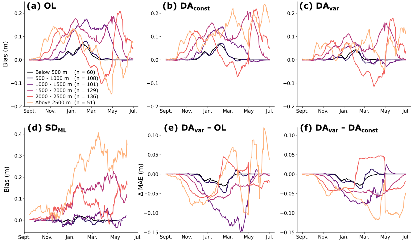
Figure 4. Seasonal evolution of bias and mean absolute error (MAE) stratified by elevation. Panels (a)–(d) show the seasonal snow depth bias for the (a) OL, (b) DA_{const} , and (c) DA_{var} experiments, and for (d) the assimilated observations ( SD_{ML} ). Bias is computed relative to in-situ snow depth measurements and is grouped by elevation bands (indicated by different colors). Panels (e)–(f) show the change in MAE between the OL and DA_{var} experiments (e) and between the DA_{const} and DA_{var} experiments (f). Negative values in (e)–(f) indicate improved performance (decreased MAE). Statistics are computed for each day, averaged over the entire 8-year period (2015–2023). A 14-day smoothing is applied to each timeseries and the number of in-situ measurement sites ( n ) within each elevation band is provided in the legend.
