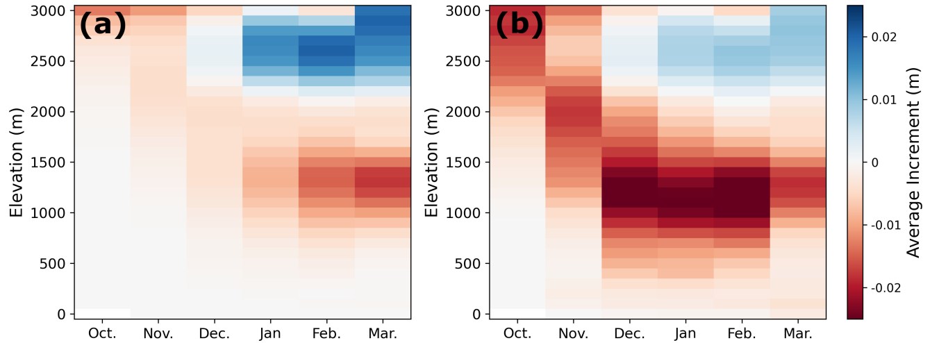
Figure 9. Average total snow depth increments (m) over the accumulation season (x-axis), stratified by elevation (y-axis) for (a) DA_{const} and (b) DA_{var} . Increments are averaged over all years (2015-2023)
