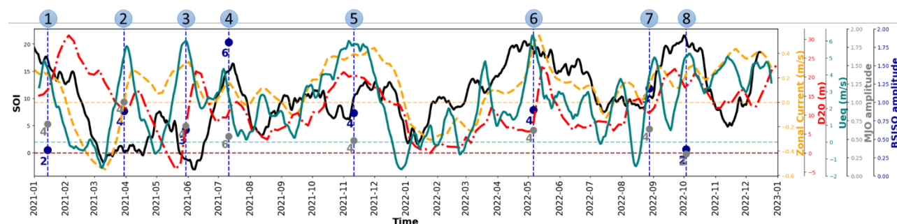
Figure 5: The time evolution of 31-day running mean of daily SOI, equatorial zonal currents (OSCAR, 2°S-2°N, 40°E-100°E), GODAS D20 anomalies over the IOD east pole, and the 10 m zonal wind anomalies (5°S-5°N, 60°E-90°E). The vertical dotted lines in blue indicate the occurrences of WWBs, and the MJO (gray)/BSISO (blue) phases on the day of WWBs are indicated by markers.
