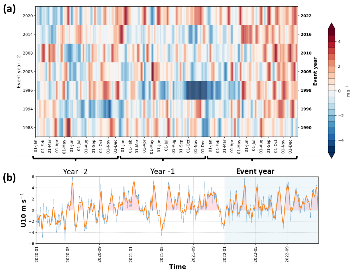
125 Figure 2: (a) The 11-day running mean of equatorial (averaged over 5°S-5°N, 60°E-90°E) 10m zonal-wind anomalies for all the nIOD events since 1980. The wind anomalies for the previous two years are indicated by Year -2 and Year -1 on the x-axis. (b) Evolution of the equatorial 10m zonal-winds wind anomalies (dashed line), its 7-day running mean (solid line) for the period January 2020 to December 2022.
