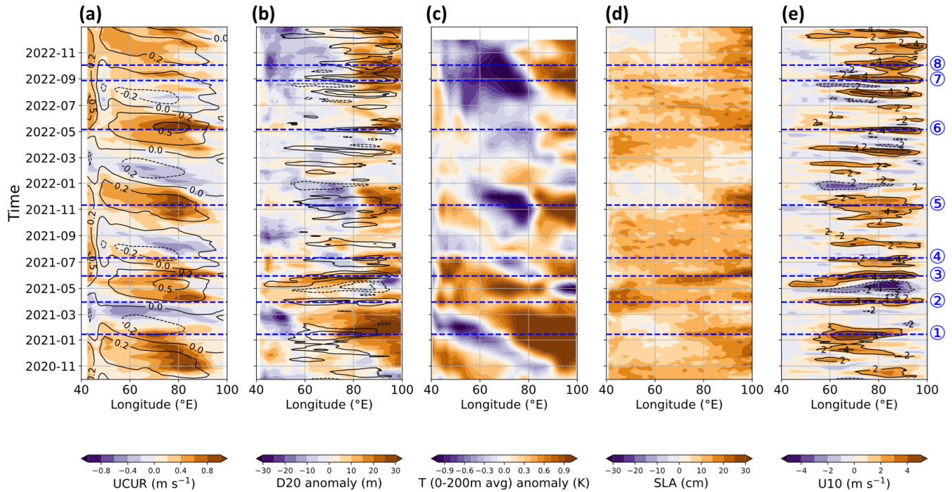
Figure 4: The time-longitude sections of (a) 2°S-2°N averaged zonal currents in the upper ocean (0-100m averaged) for 40°E-100°E along with the climatological currents (contours), (b) The D20 anomaly (m) from NCEP GODAS (shading), and the 11-day running mean of 10 m zonal wind anomaly ( \text{m s}^{-1} ) averaged over 5°S-5°N (positive (negative) values are indicated by solid (dashed) contours and the contour interval is -4 to 4 by 2, zero contour is not shown), (c) the 0-200m averaged weekly temperature anomaly from NCEP GODAS, (d) the observed sea-level anomaly (SLA) from AVISO, and (e) 11-day running mean of zonal wind (shading) and zonal wind anomaly (contours).
