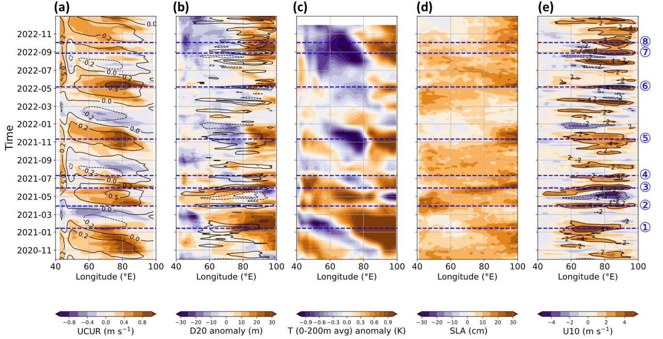
195 Figure 4: The time-longitude sections of (a) 2°S-2°N averaged zonal currents in the upper ocean (0-100m averaged) for 40°E-100°E along with the climatological currents (contours) obtained from OSCAR, (b) The D20 anomaly (m) from NCEP GODAS (shading), and the 11-day running mean of 10 m zonal wind anomaly ( \text{m s}^{-1} ) averaged over 5°S-5°N (positive (negative) values are indicated by solid (dashed) contours and the contour interval is -4 to 4 by 2, zero contour is not shown), (c) the 0-200m averaged weekly temperature anomaly from NCEP GODAS, (d) the observed 200 Altimeter satellite gridded Sea Level Anomaly (SLA) level 4 data obtained from the Copernicus Marine Service website, and (e) 11-day running mean of zonal wind (shading) and zonal wind anomaly (contours).
