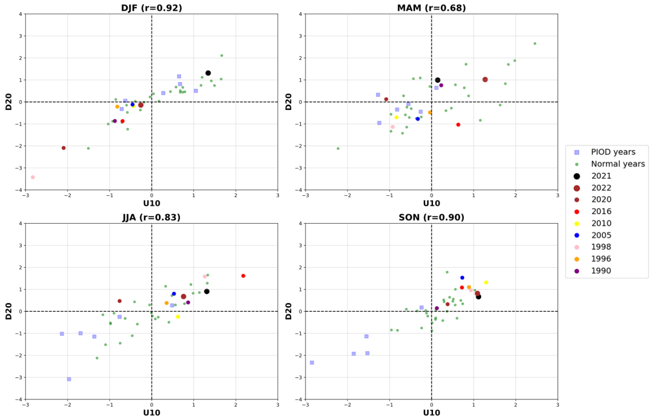
335 Figure 8: Scatter plot of the standardized anomalies of 10 m zonal winds over the equator (U10; averaged over 5°S-5°N, 60°E-90°E) and D20 anomalies over the IOD east pole region for different seasons. The correlation (r) between the time series is indicated in brackets.
