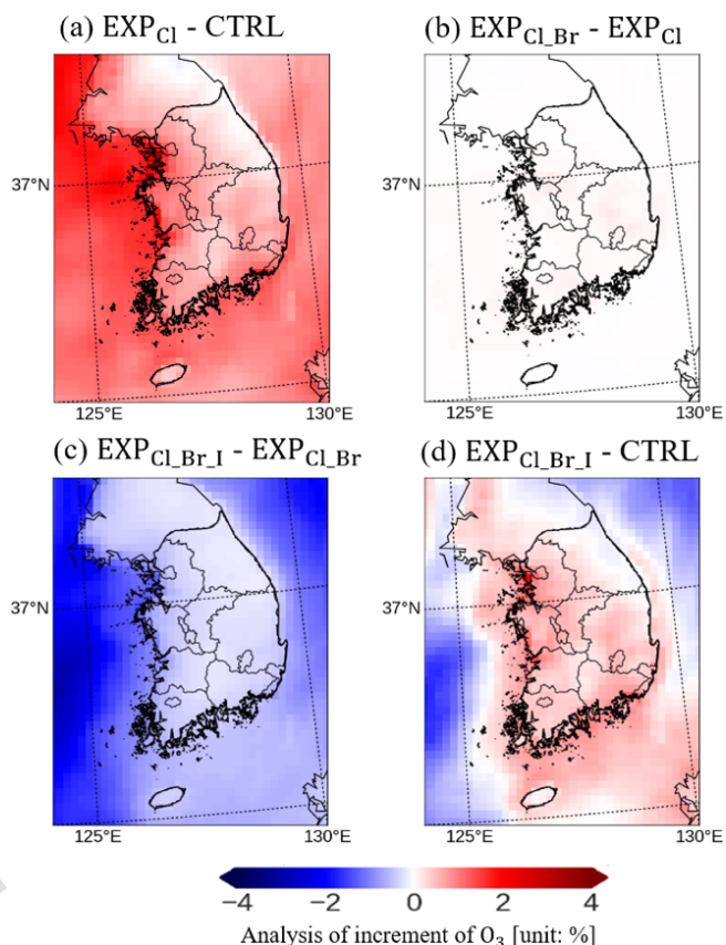
Figure 7. Spatial impacts of (a) chlorine processes ( EXP_{Cl} - CTRL ), (b) bromine processes ( EXP_{Cl\_Br} - EXP_{Cl} ), (c) iodine processes ( EXP_{Cl\_Br\_I} - EXP_{Cl\_Br} ), and (d) total halogen processes ( EXP_{Cl\_Br\_I} - CTRL ) on O_3 mixing ratios over the Korean Peninsula.
