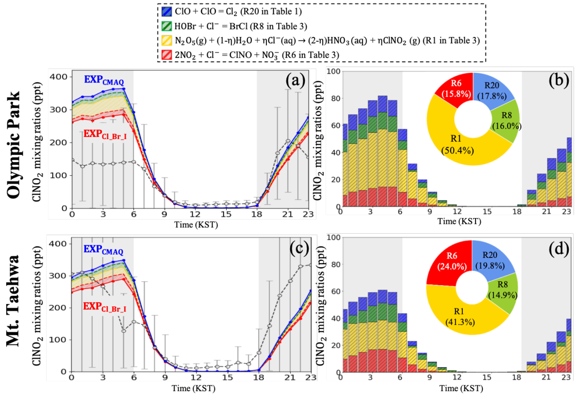
Figure 3. Contributions of halogen reactions to the mixing ratios of ClNO 2 in the EXP CMAQ and EXP Cl 2 Br 2 I simulations at (a and b) Olympic Park and (c and d) Mt. Taehwa stations during the period of KORUS-AQ campaign. Stacked bars and pie charts show the contributions from four halogen reactions to the mixing ratios of ClNO 2 . Grey-shaded areas represent nighttime (18:00-06:00 local standard time).
