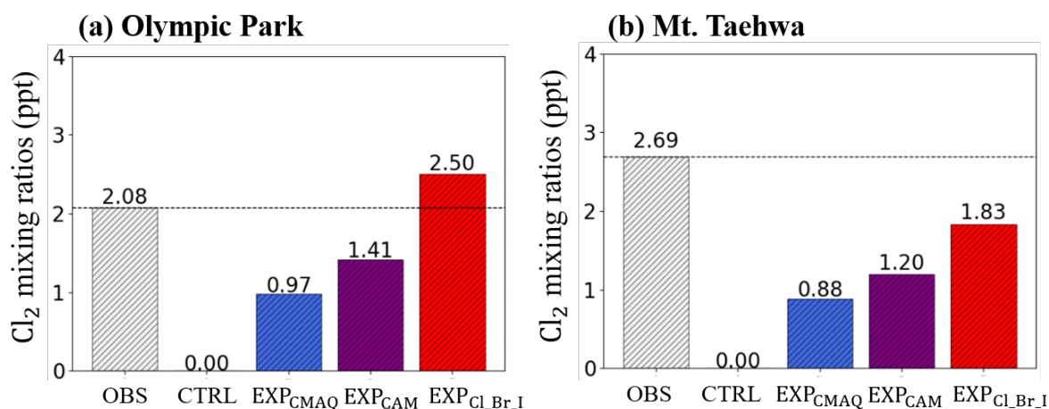
Figure 4. Comparisons of averaged mixing ratios of \text{Cl}_2 observed (OBS) and modeled from four simulations (CTRL, \text{EXP}_{\text{CMAQ}} , \text{EXP}_{\text{CAM}} , and \text{EXP}_{\text{Cl}_\text{Br}_\text{I}} ) at (a) Olympic Park and (b) Mt. Taehwa stations. Dotted lines represent the observed mixing ratios of \text{Cl}_2 .
