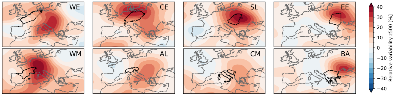
Figure 5. Relative variability of z500 anomaly during SCO compared to the rest of the analyzed period in each region
