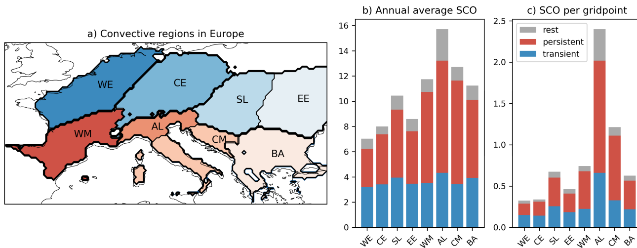
Figure 1. Identified convective regions with K-means clustering and their convective activity. Panel b) shows the number of annual SCO per aggregated region, panel c) shows the total number of SCO per regional grid point.
