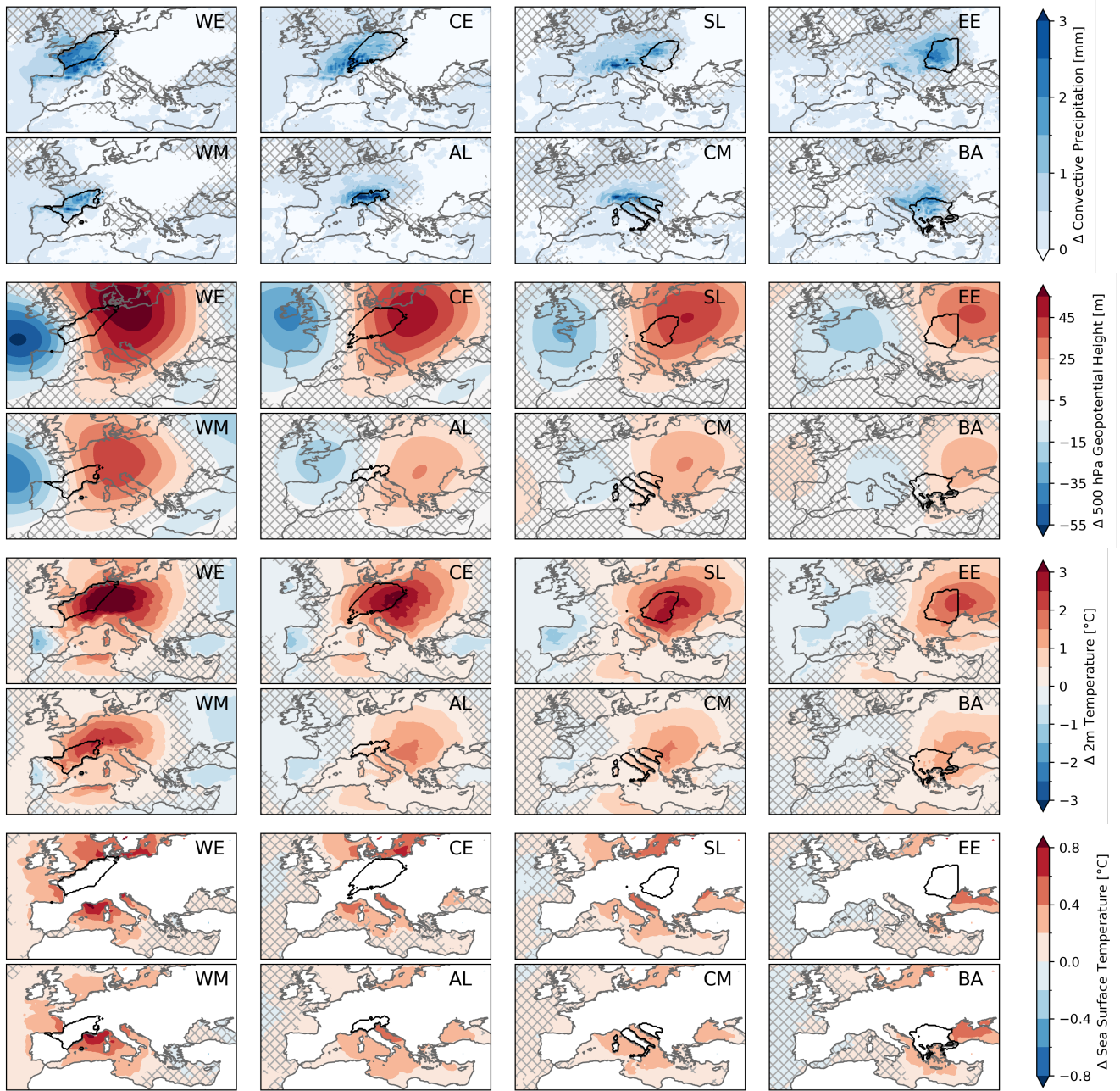
Figure 4. Synoptic anomalies on first day of SCO. The number of SCO per region is depicted in Fig. 1b. Hatching is applied to non-significant areas. The convective region is outlined in black and labelled in the top-right of each panel.
