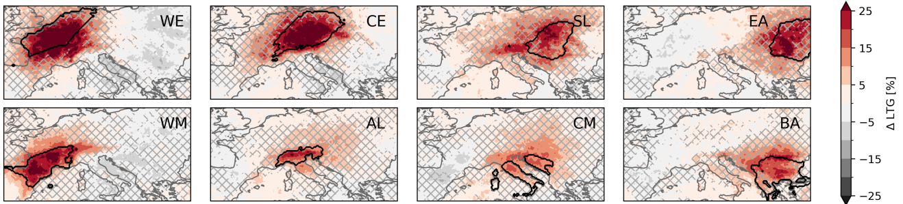
Figure 3. Anomaly of lightning presence on first day of SCO. The number of SCO per region is depicted in Fig. 1b. Hatching is applied to non-significant areas. The convective region is outlined in black and labelled in the top-right of each panel.
