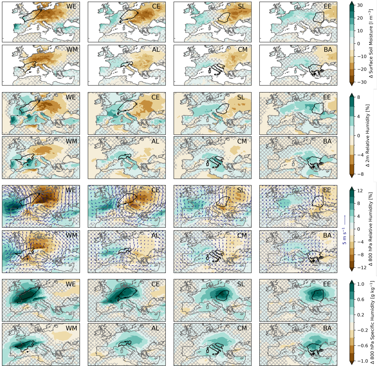
Figure 6. Moisture anomalies on first day of SCO. The number of SCO per region is depicted in Fig. 1b. Hatching is applied to non-significant areas. The convective region is outlined in black and labelled in the top-right of each panel. Arrows over 800 hPa relative humidity indicate wind at 800 hPa.
