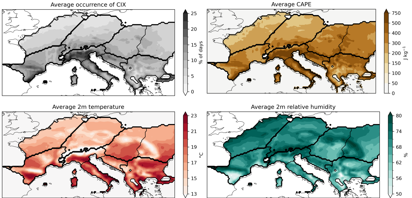
Figure 2. Climatological mean convective activity, CAPE, 2m temperature, and 2m relative humidity
