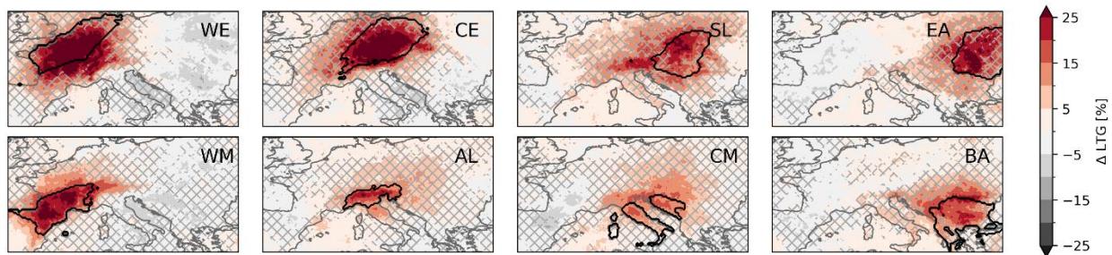
Fig. R3: Anomaly of lightning activity on first day of SCO per region.
