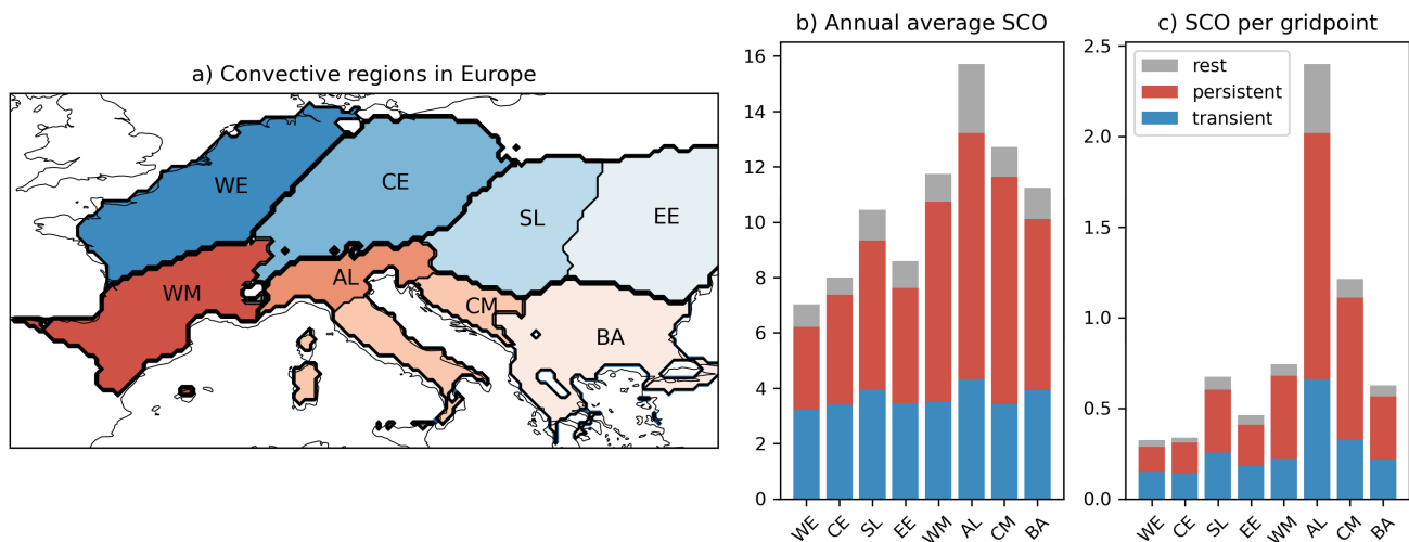
Figure 1. Identified convective regions with K-means clustering and their convective activity. Panel b) shows the total number of annual SCO per regional-grid-point aggregated region , panel c) shows the total number of annual SCO per aggregated-region regional grid point .
