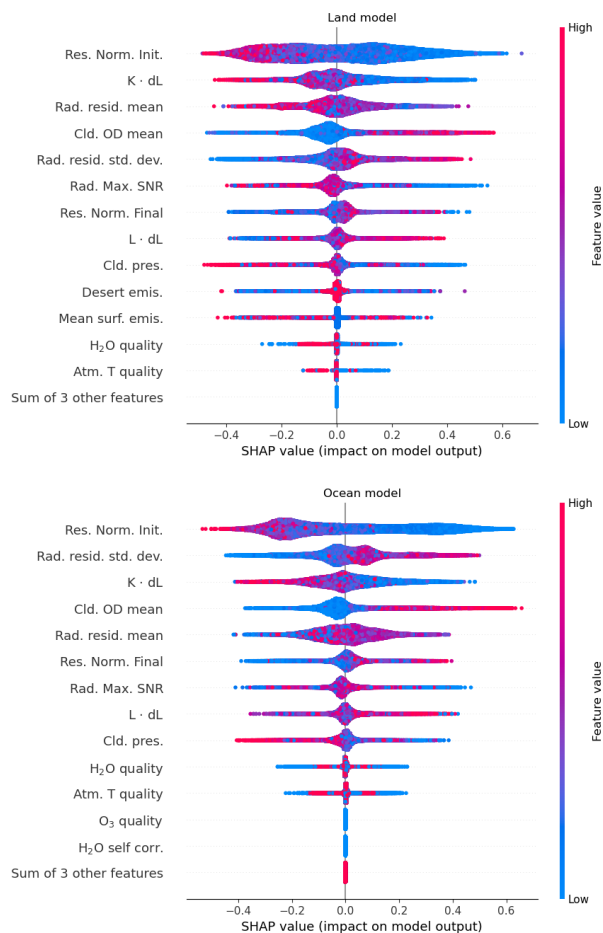
Figure A1. Beeswarm plot showing the Shapley values for the 13 input variables for the quality filtering decision trees that have non-zero contributions to the output flag. The meaning of each input variable’s short name is given in Table 5.
