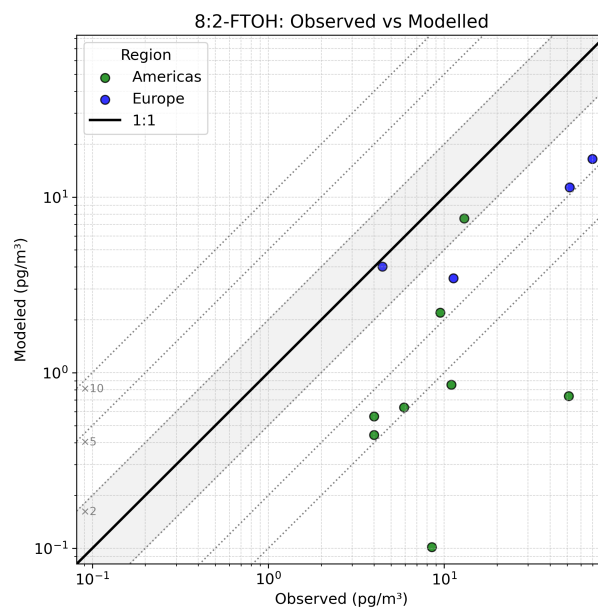
Figure D3. Comparison of observed versus modeled 8:2 FTOH concentrations ( \text{pg m}^{-3} ) by region on a log-log scale. The solid line represents 1:1 agreement, with dotted lines indicating deviations by factors of 2, 5, and 10.
