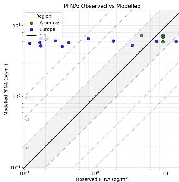
Figure D2. Comparison of observed versus modeled PFNA concentrations ( \text{pg m}^{-3} ) by region on a log-log scale. The solid line represents 1:1 agreement, with dotted lines indicating deviations by factors of 2, 5, and 10 .
