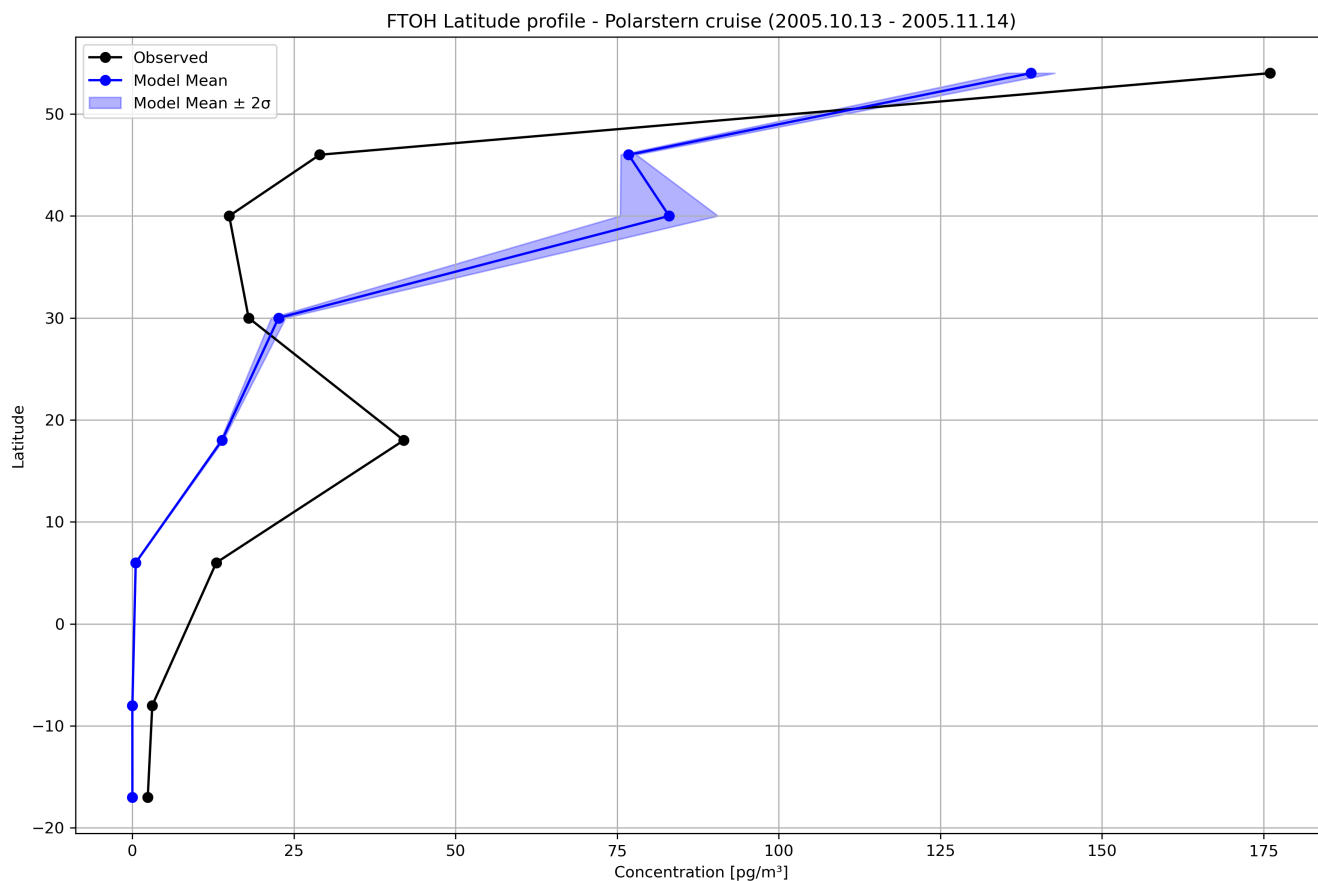
Figure 6. 8:2 FTOH latitudinal profile of atmospheric concentrations [ \text{pg}/\text{m}^3 ]. Observed data (black) vs. Model (blue line). The shaded blue area indicates the model variability, defined as \pm 2 standard deviations calculated over the sampling period.
