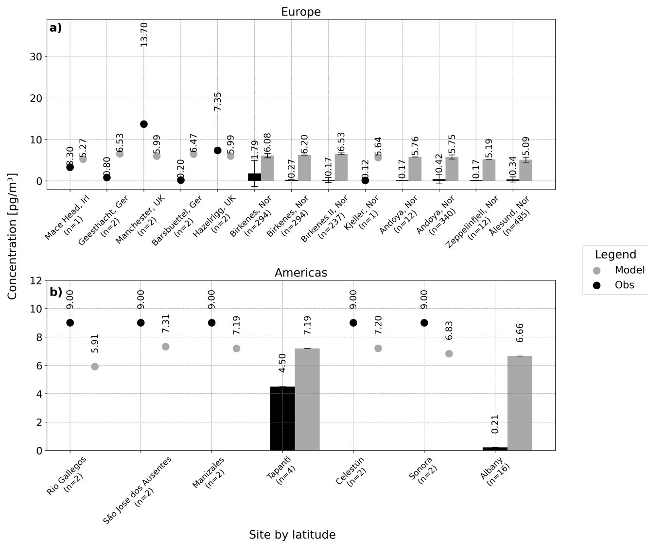
Figure 4. PFNA observed and simulated atmospheric concentrations [ \text{pg}/\text{m}^3 ] in Europe and the Americas. Observed (black), Modeled (gray). Number of observations next to site.
