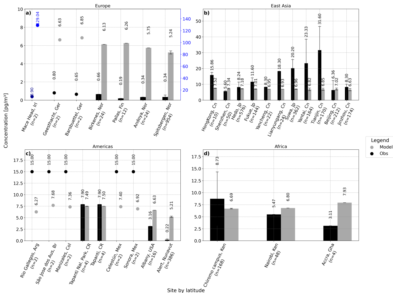
Figure 2. Observed and simulated atmospheric PFOA concentrations [pg/m 3 ] in a) Europe, b) East Asia, c) Americas and d) Africa. Observed (black), modeled (gray) and number of observations (down the site name). Panel (a) includes a secondary right-hand axis (blue) for the Mace Head site, due to its large magnitude values.
