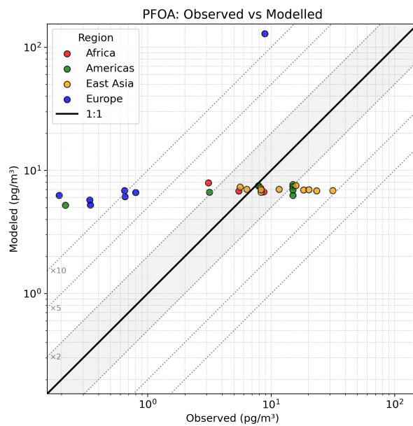
Figure D1. PFOA Comparison of observed vs modeled factor plot PFOA concentrations ( pg m -3 ) by region on a log-log scale. The solid line represents 1:1 agreement, with dotted lines indicating deviations by factors of 2, 5, 5 and 10 10
