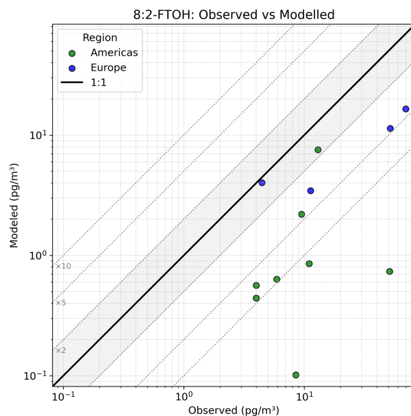
Figure D3. Comparison of observed versus modeled 8:2 FTOH observed-vs-modeled-factor-plot concentrations ( \times 2 \text{ pg m}^{-3} ) by region on a log-log scale. The solid line represents 1:1 agreement, with dotted lines indicating deviations by factors of 2, 5, \times 5 and \times 10 10.
