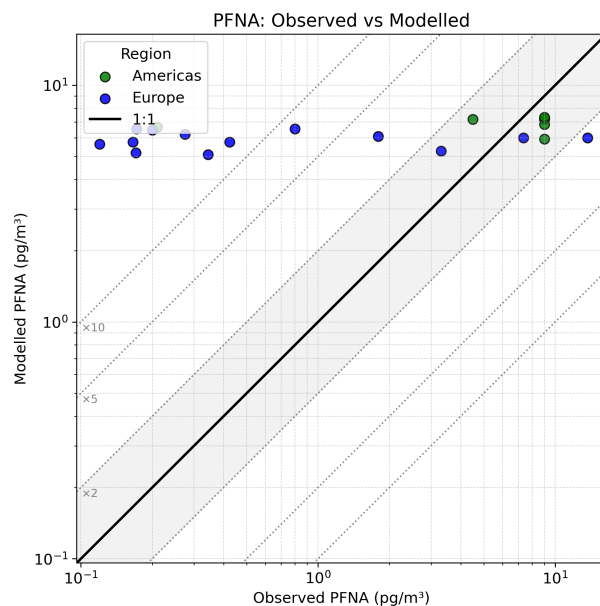
Figure D2. PFNA: Comparison of observed vs versus modeled factor-plot PFNA concentrations ( \times 2 \text{ pg m}^{-3} ) by region on a log-log scale. The solid line represents 1:1 agreement, with dotted lines indicating deviations by factors of 2, 5, \times 5 and \times 10 10 .
