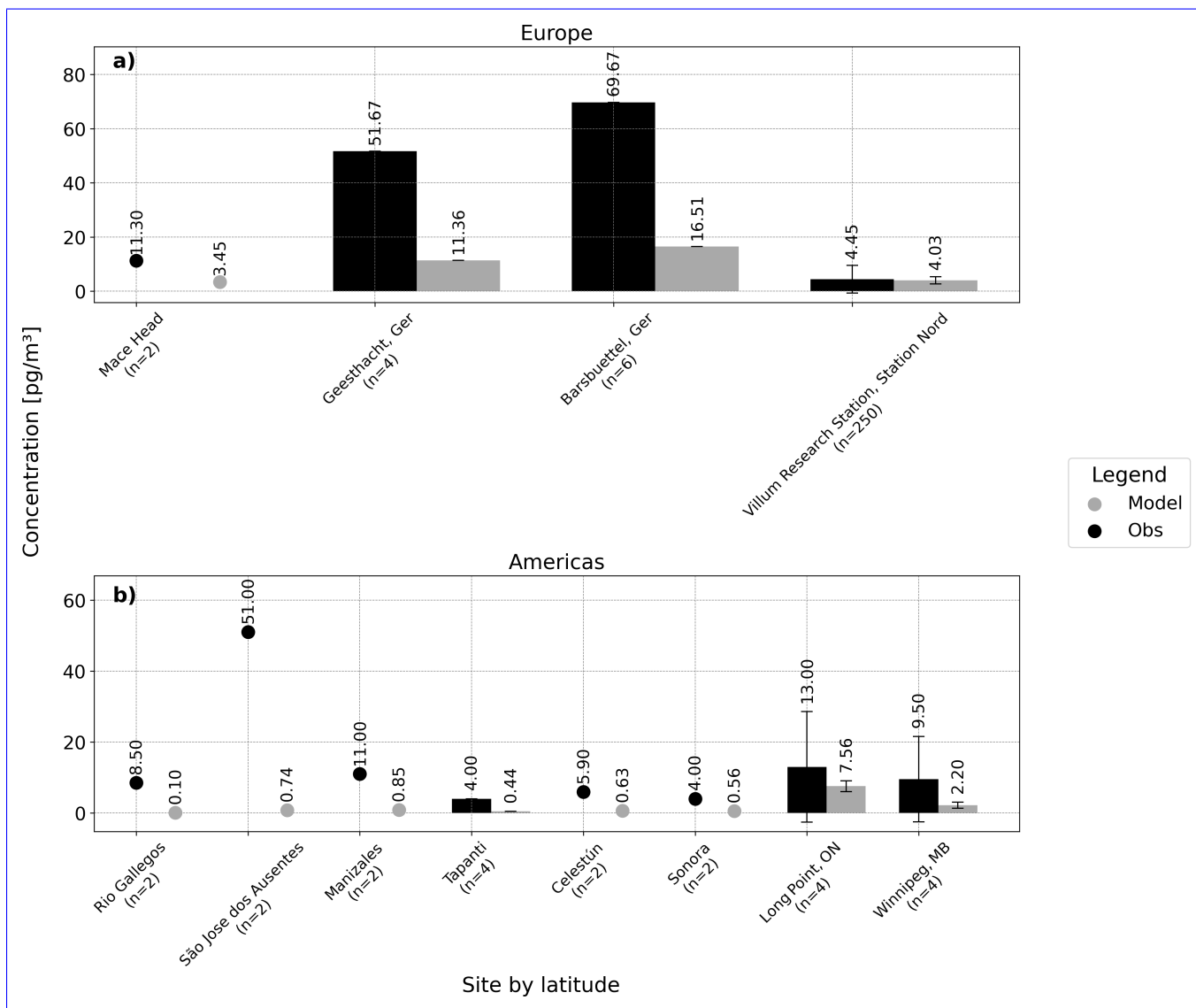
Figure 3. Observed and simulated atmospheric FTOH concentrations [ \text{pg}/\text{m}^3 ] in Europe and the Americas. Observed (black), modeled (gray) and number of observations.
