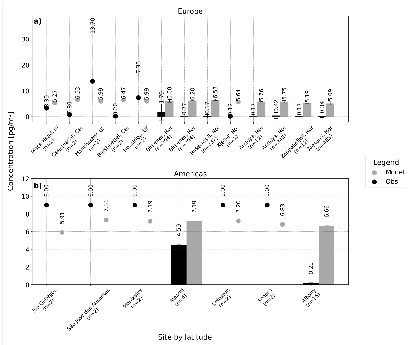
Figure 4. PFNA observed and simulated atmospheric concentrations [ \text{pg}/\text{m}^3 ] in Europe and the Americas. Observed (black), Modeled (gray). Number of observations next to site.
