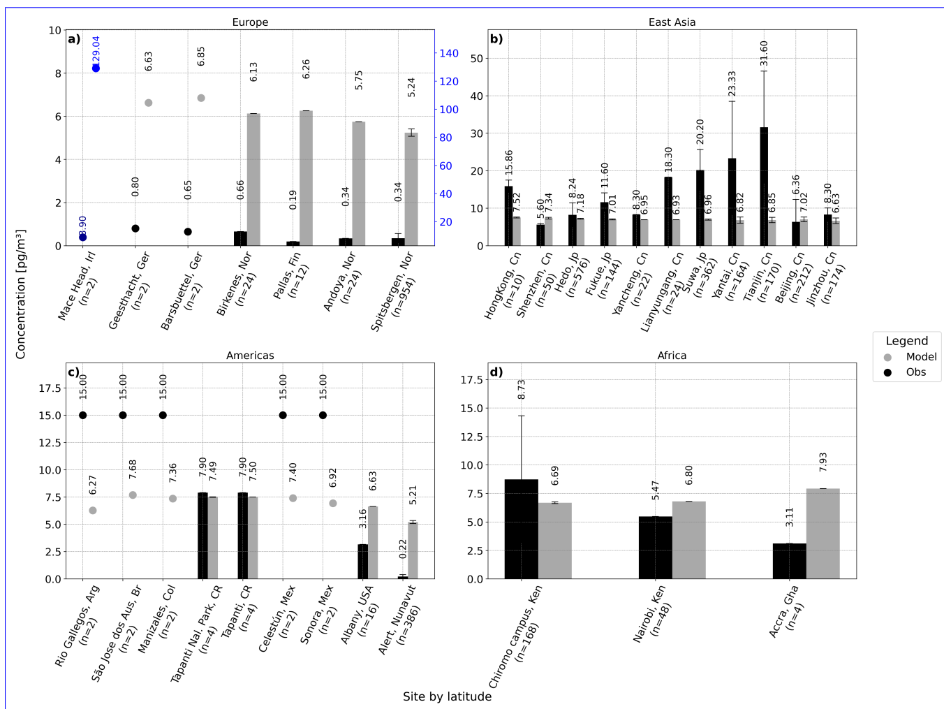
Figure 2. Observed and simulated atmospheric PFOA concentrations [ \text{pg}/\text{m}^3 ] in a) Europe, b) East Asia, c) Americas and d) Africa. Observed (black), modeled (gray) and number of observations (down the site name). Panel (a) includes a secondary right-hand axis (blue) for the Mace Head site, due to its large magnitude values.
