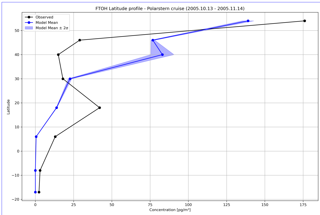
Figure 6. 8:2 FTOH latitudinal profile of atmospheric concentrations [pg/m 3 ]. Observed data (black) vs. Model (blue line). The shaded blue area indicates the model variability, defined as \pm 2 standard deviations calculated over the sampling period.
