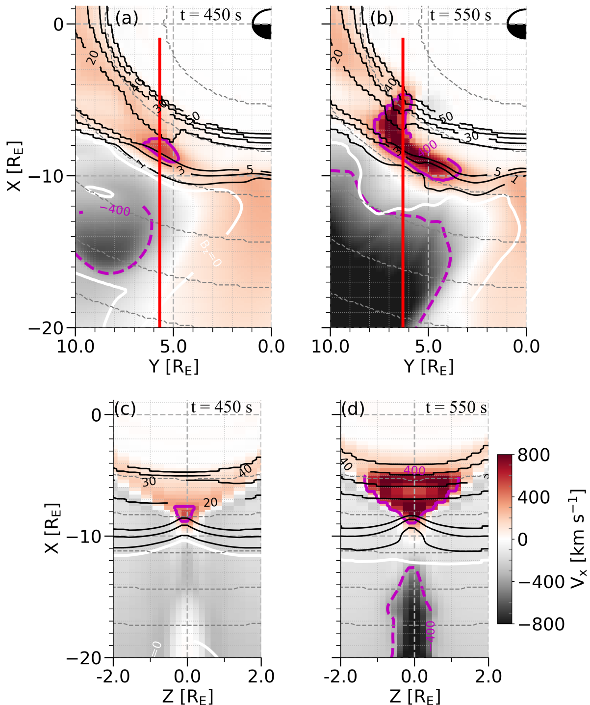
Figure 2. (a, b) Same as Figures 1d and 1j at simulation times t=450 s and t=550 s, respectively, but showing only the duskside magnetotail in the XY plane at Z=0 . (c, d) Snapshots of the x-component of the flow velocity V_x in the XZ plane at Y = 5.7 R_E and Y = 6.3 R_E as indicated by the red vertical lines on panels (a) and (b)
