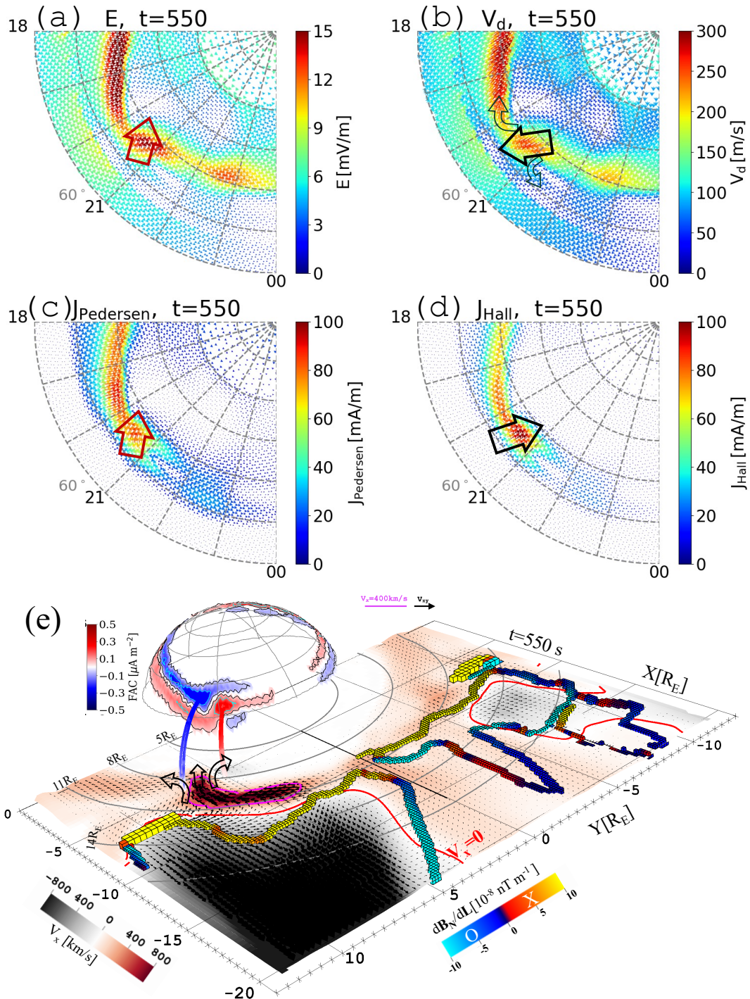
Figure 7. (a) Ionospheric electric field E , (b) plasma drift velocity V_d , (c) Pedersen current J_{Pedersen} , (d) Hall current J_{Hall} and (e) magnetic conjugacy of ionosphere and FACs associated with BBF, and plasma flow pattern on the dawn- and dusksides of the BBF in the current sheet at simulation time t = 550 s. The colourmap on the current sheet shows the x-component of velocity.
