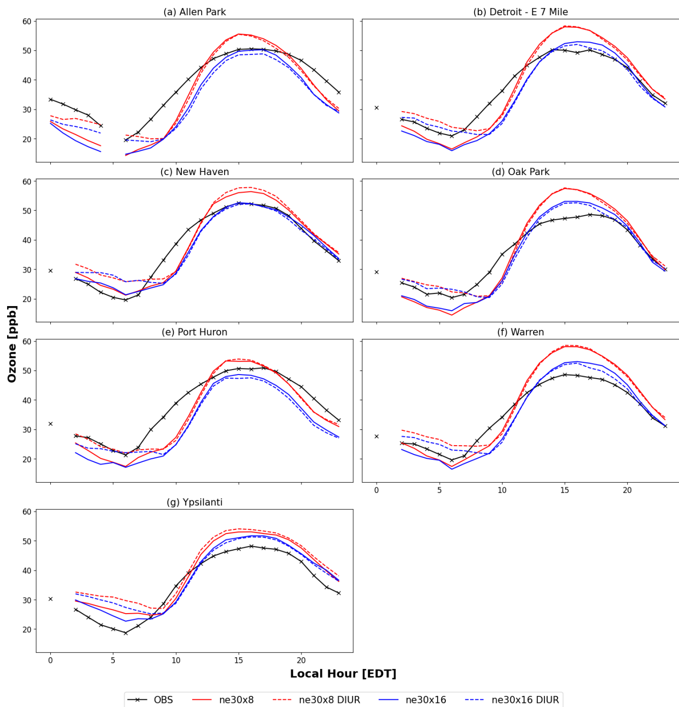
337 Figure 4: Model evaluation of hourly averaged diurnal profiles of ozone concentrations at the surface during the Michigan-Ontario 338 Ozone Source Experiment (24 May to 30 June 2021) at seven stationary measurement sites in Southeast Michigan – a) Allen Park 339 [42.2°N, 276.8°W]; b) Detroit – E 7 Mile [42.4°N, 277.0°W]; c) New Haven [42.7°N, 277.2°W]; d) Oak Park [42.5°N, 276.8°W]; e) Port
