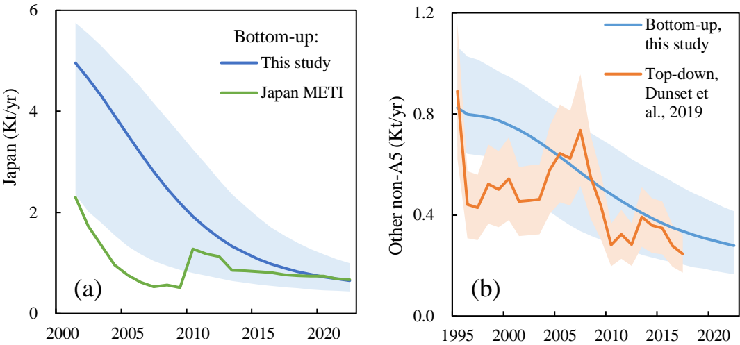
Figure S14 Comparison of CFC-11 emissions in Japan (a) and other non-A5 parties (b)
