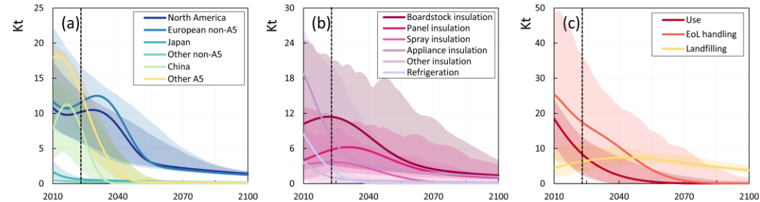
Figure S15 Banked CFC-11 emissions categorized by region (a), sector (b), and life stage (c)
