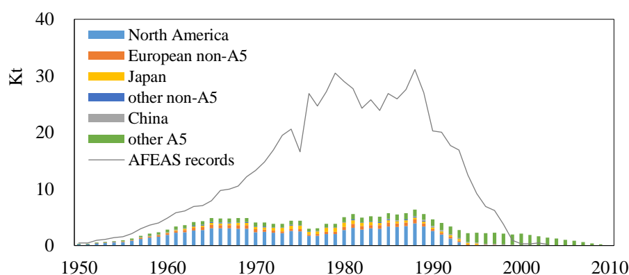
Figure S10 Estimation of CFC-11 consumption in new refrigeration systems across various regions, compared with CFC-11 sales data in non-hermetic refrigeration systems recorded by AFEAS (2003)
