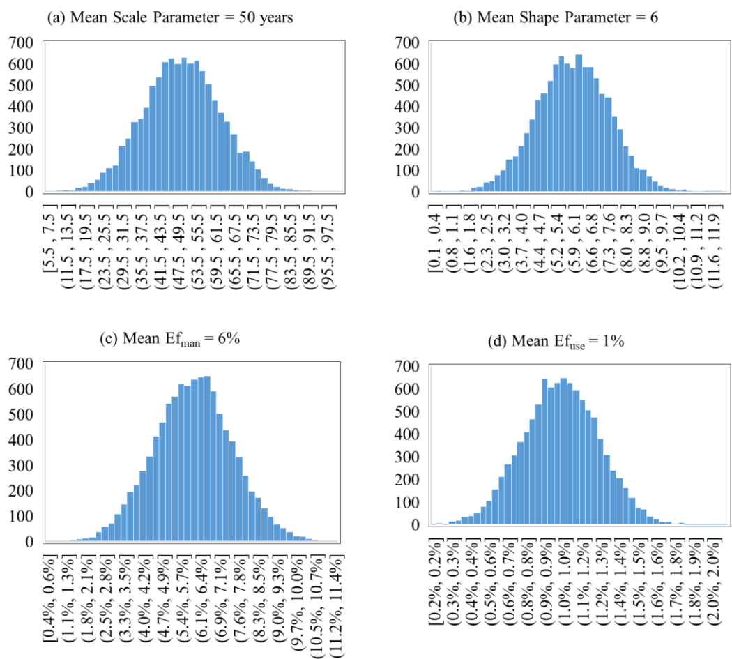
Figure S13 Distribution of key parameters in this study: Weibull scale (a) and shape parameters (b), along with emission factors during the manufacturing (c) and use stage (d) for polyurethane rigid boardstock/laminate foam products. N=10^4
