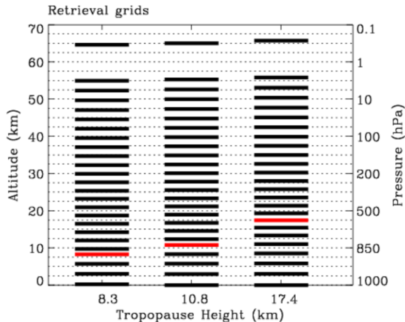
Figure S1. The 25 pressure levels used to retrieve partial ozone columns at 24 layers for three different atmospheric profiles, each with a different tropopause height (noted along the x-axis). The initial vertical pressure grid is defined as P_i = 2^{-i/2} atm for i = 0 to 23, with the top-of-atmosphere pressure set at P_{24} . This grid is then adjusted by replacing the levels nearest to the surface pressure and thermal tropopause pressure. Tropospheric layers are redistributed evenly in logarithmic pressure space. Typically, 3 to 7 layers are assigned within the troposphere region.
