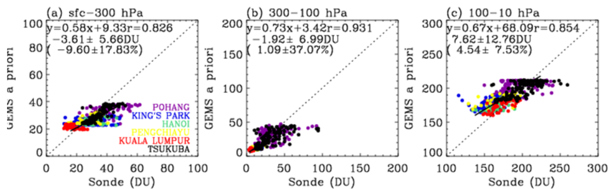
Figure S4. Same as Figure 11, but for scatters between GEMS a priori and ozonesonde measurements. The a priori is taken from tropopause-based ozone profile climatology (Bak et al. 2013).
