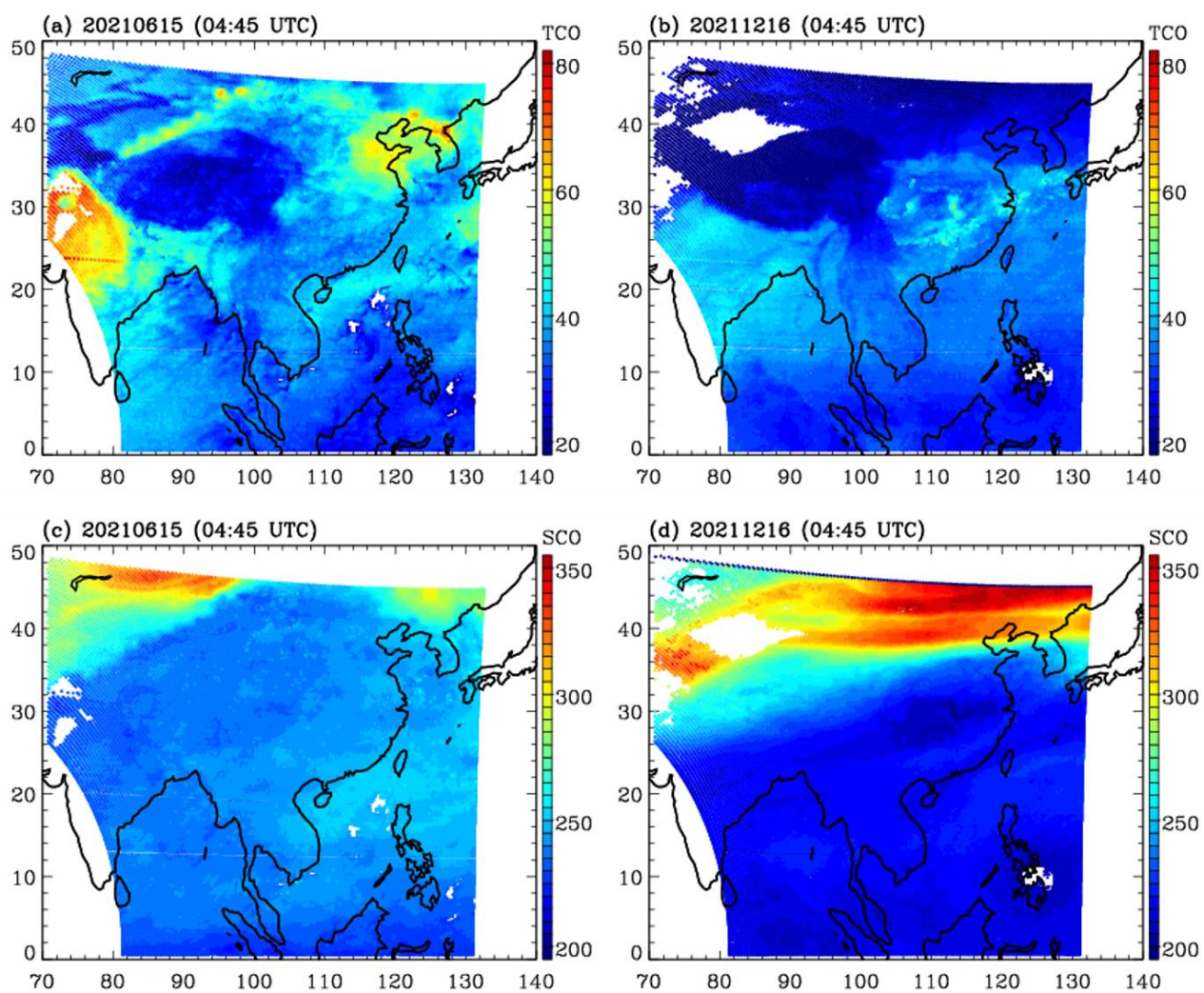
Figure S2. Tropospheric and stratospheric column ozone distribution on 15 June and 16 December 2021 (04:45 UTC).
