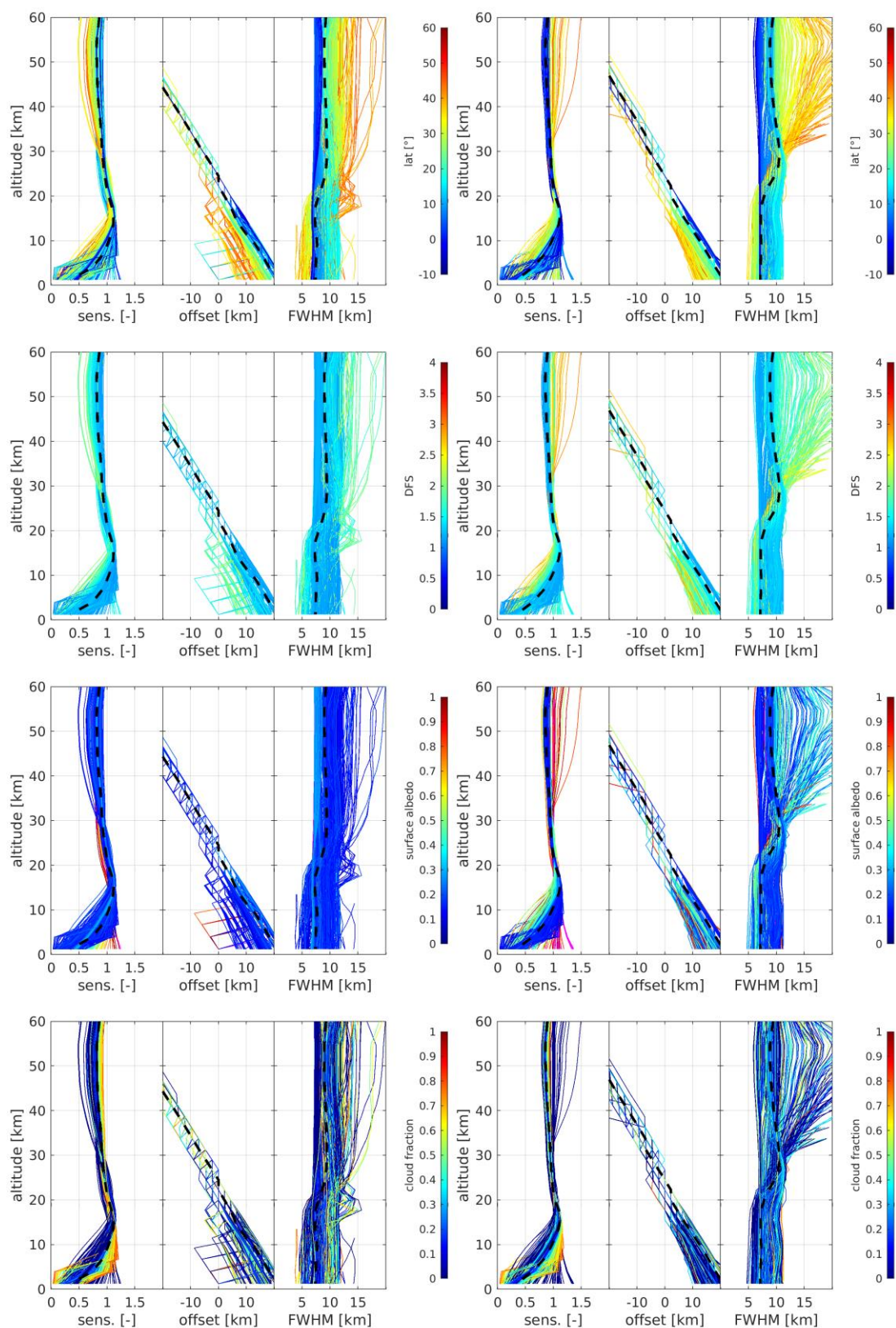
Figure S2. GEMS ozone profile retrieval information content in terms of sensitivity, offset, and kernel FWHM for 15 June (left) and 16 December (right) 2021, and for four major influence quantities (top to bottom), color-coded in each plot. Median values are indicated by black dashed lines.
