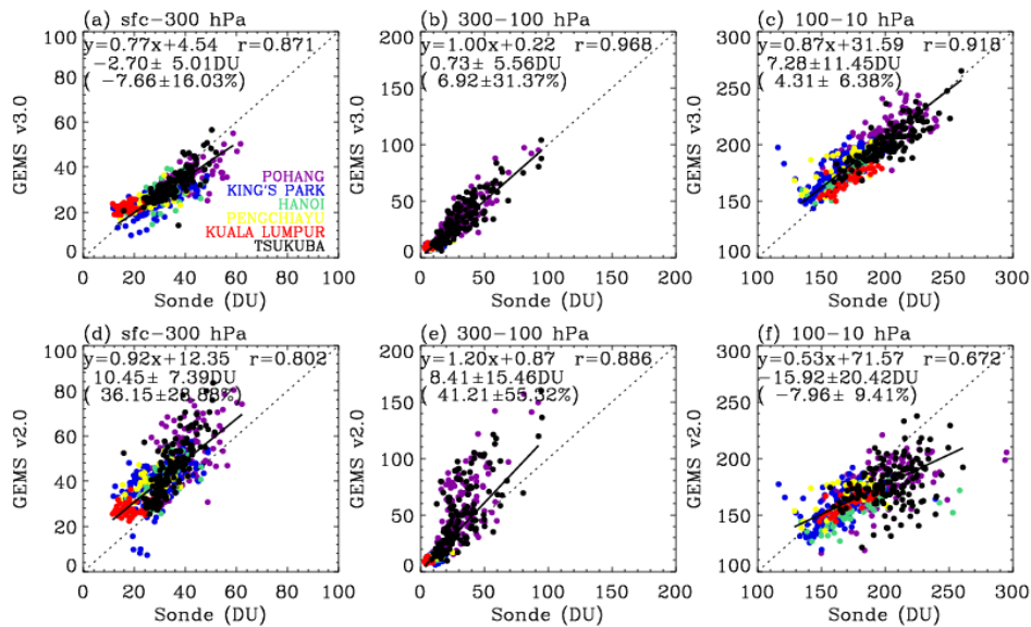
417 418 Figure 11. Scatter plots of GEMS and ozonesonde ozone columns for three different layers, surface-300 hPa, 300-100 419 hPa, and 100-10 hPa. The upper (a-c) panels show results from GEMS v3.0, and the bottom panels (d-f) from GEMS
