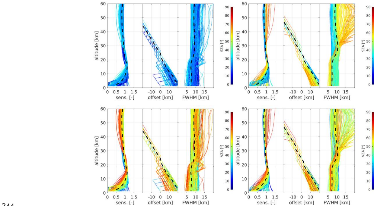
344 Figure 8: Sensitivity, offset, and kernel FWHM for GEMS ozone profile retrievals on June 15 (left) and December 16 345 (right) 2021. Black dashed lines indicate median values. Color coding represents SZA (top) and VZA (bottom), which 346 are the primary quantities influencing retrieval characteristics; additional factors are presented in the Supplement. 347
