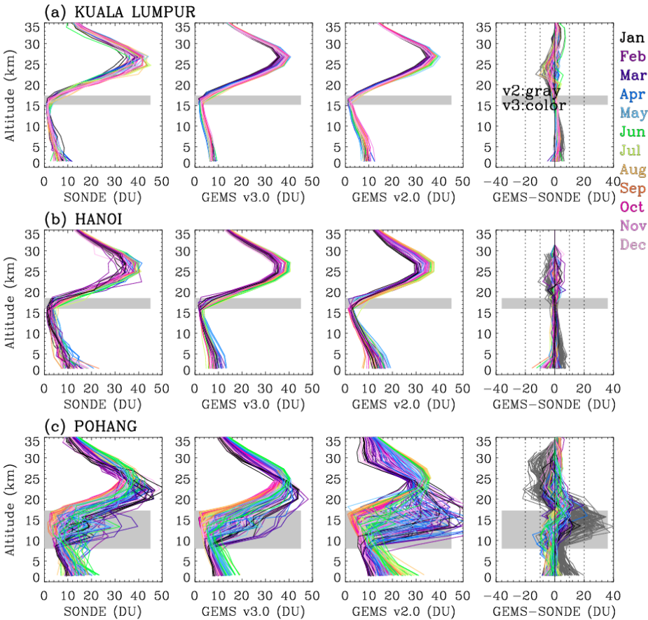
373 Figure 9. Ozone vertical profiles (in DU) at three sites—(a) Kuala Lumpur, (b) Hanoi, and (c) Pohang—during 2021– 374 2024. Each panel displays individual ozonesonde soundings along with corresponding GEMS v3.0 and v2.0 retrievals. 375 The last columns present the respective differences (GEMS – SONDE) for GEMS v3.0 and v2.0, displayed in color and 376 dark gray, respectively. The gray shaded area denotes the range of tropopause altitudes (minimum to maximum).
