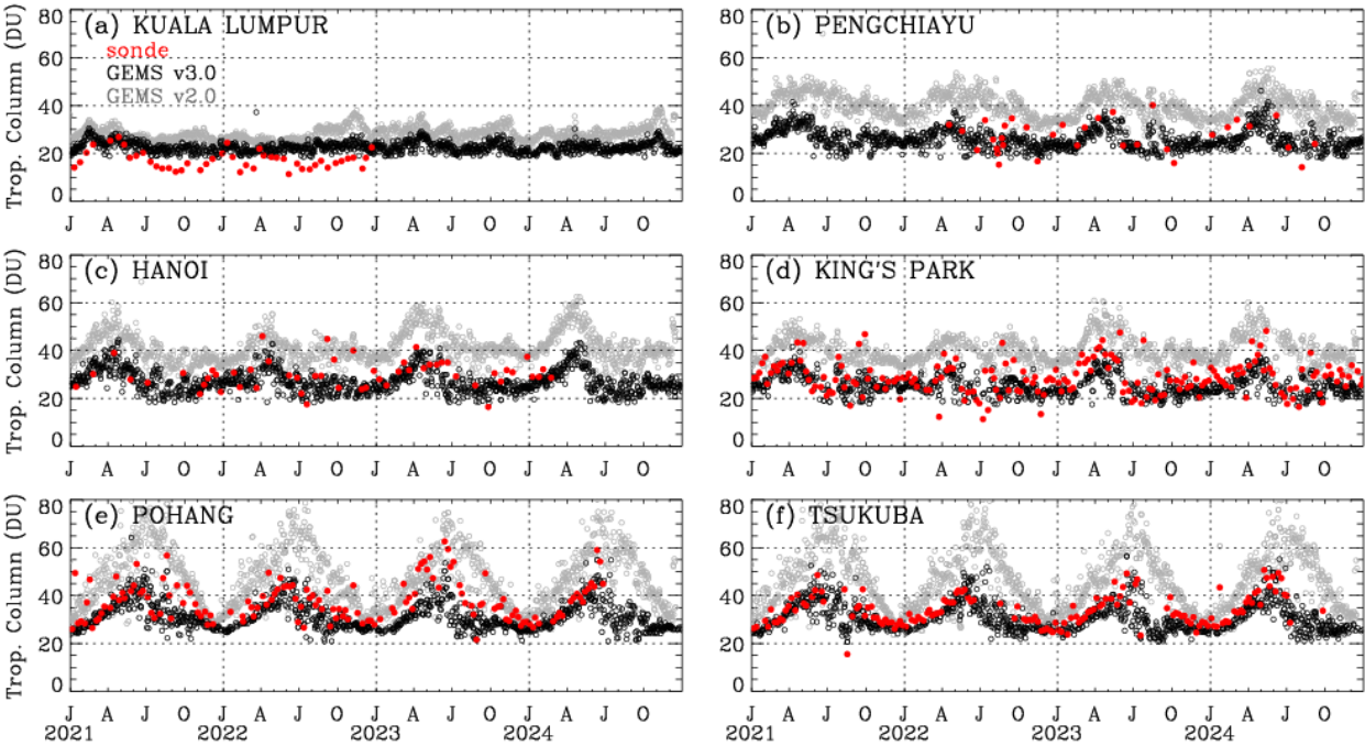
393 394 Figure 10. Time-series of tropospheric ozone columns (surface-300 hPa) from GEMS v3.0 (black), GEMS v2.0 (grey), 395 and ozonesondes (red). The x-axis marks the months of the year using initials: J (January), A (April), J (July), and O 396 (October).
