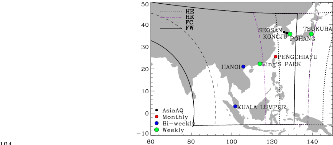
104 105 Figure 1. Geographic coverage of the four GEMS scan modes: Half East (HE), Half Korea (HK), Full Central (FC), 106 and Full West (FW), indicated by the curved boundaries. Colored dots indicate ozonesonde stations with regular 107 launches within the GEMS domain, classified by launch frequency: red for monthly, blue for bi-weekly, and green for 108 weekly. Black dots represent additional sites that participated during the Asia-AQ campaign. 109
