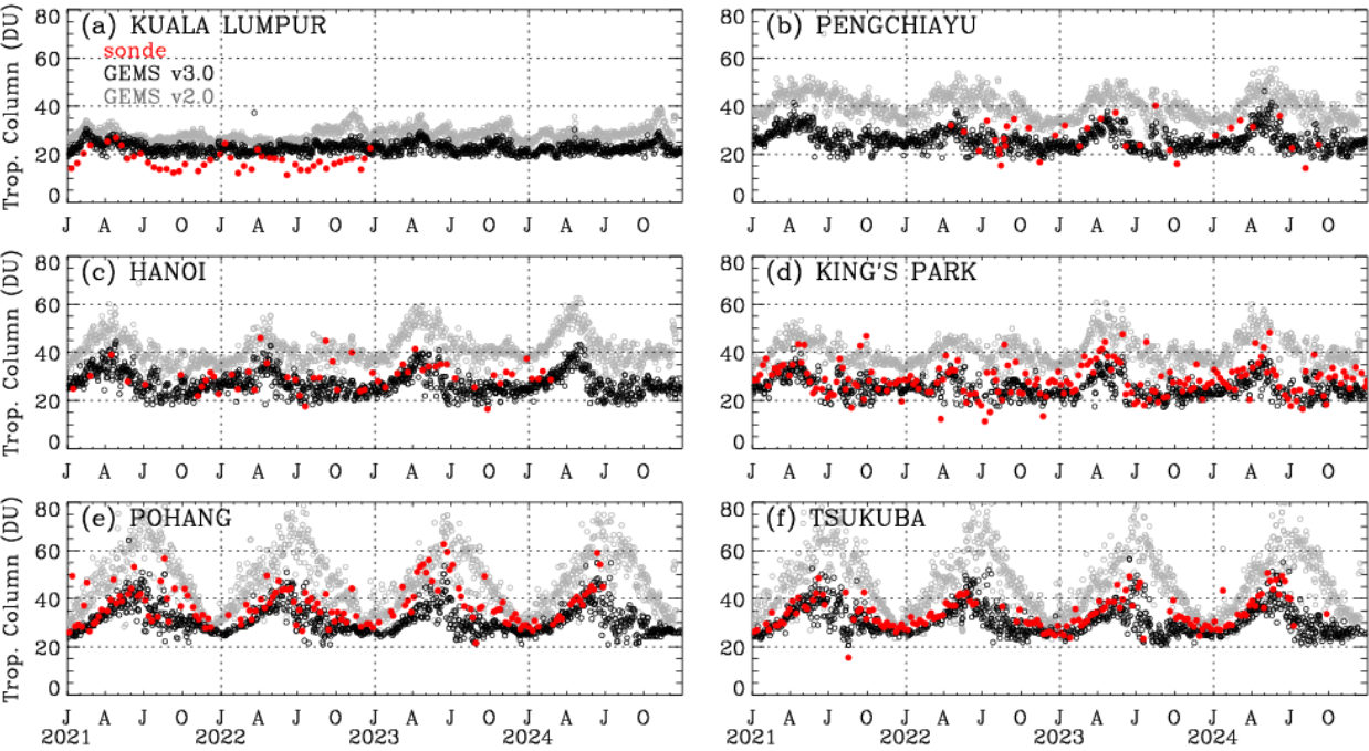
392 393 Figure 10. Time-series of tropospheric ozone columns (surface-300 hPa) from GEMS v3.0 (black), GEMS v2.0 (grey), 394 and ozonesondes (red). The x-axis marks the months of the year using initials: J (January), A (April), J (July), and O 395 (October).
