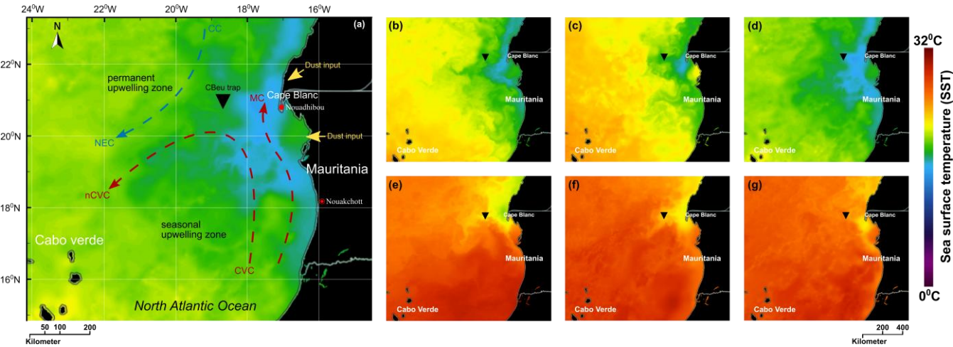
Figure 2: Location of the moored sediment trap on the Northwest African coast and temperature of the upper water column extracted from Imagery © 2025 NASA “State Of The Ocean (SOTO)”: (a) the main hydrographic currents of the Atlantic coast of Mauritania depicted after Mittelstaedt (1983, 1991) and Zenk et al. (1991) showing Canary Current (CC) and North Equatorial Current (NEC) in the blue arrow (representing colder waters) as well as Cape Verde Current (CVC), north Cape Verde Current (nCVC), and Mauritania Current (MC) in red arrows (representing warmer waters). The warmer and colder colours of the sea surface correspond to the temperature, as shown by the
