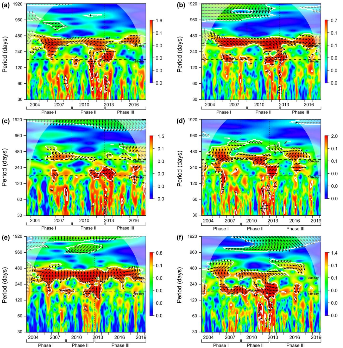
Figure 8: The wavelet cross-correlation analyses between time series of environmental parameters ( t_1 ): (a) surface wind speed, (b) surface wind direction, (c) dust storm events (Nouadhibou airport), (d) aerosol dust concentration (Cabo Verde), (e) sea surface temperature, (f) upwelling index; and total dinocyst export flux ( t_2 ). The colours of wavelet spectra indicate correlation level, white solid lines represent lines of significance, transparent grey area marks the cone of influence, vertical dashed lines indicate phase separation, and the black
