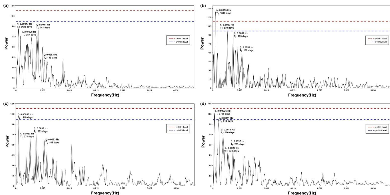
825 Figure A1: Periodogram of spectral analysis applied to the time series of total dinocysts export flux. This graph depicts the four highest frequencies ( f ) equivalent to periods ( T ) that occurred in the wavelet power spectra, of which three periodicities cross the significance line ( p < 0.05 ).
