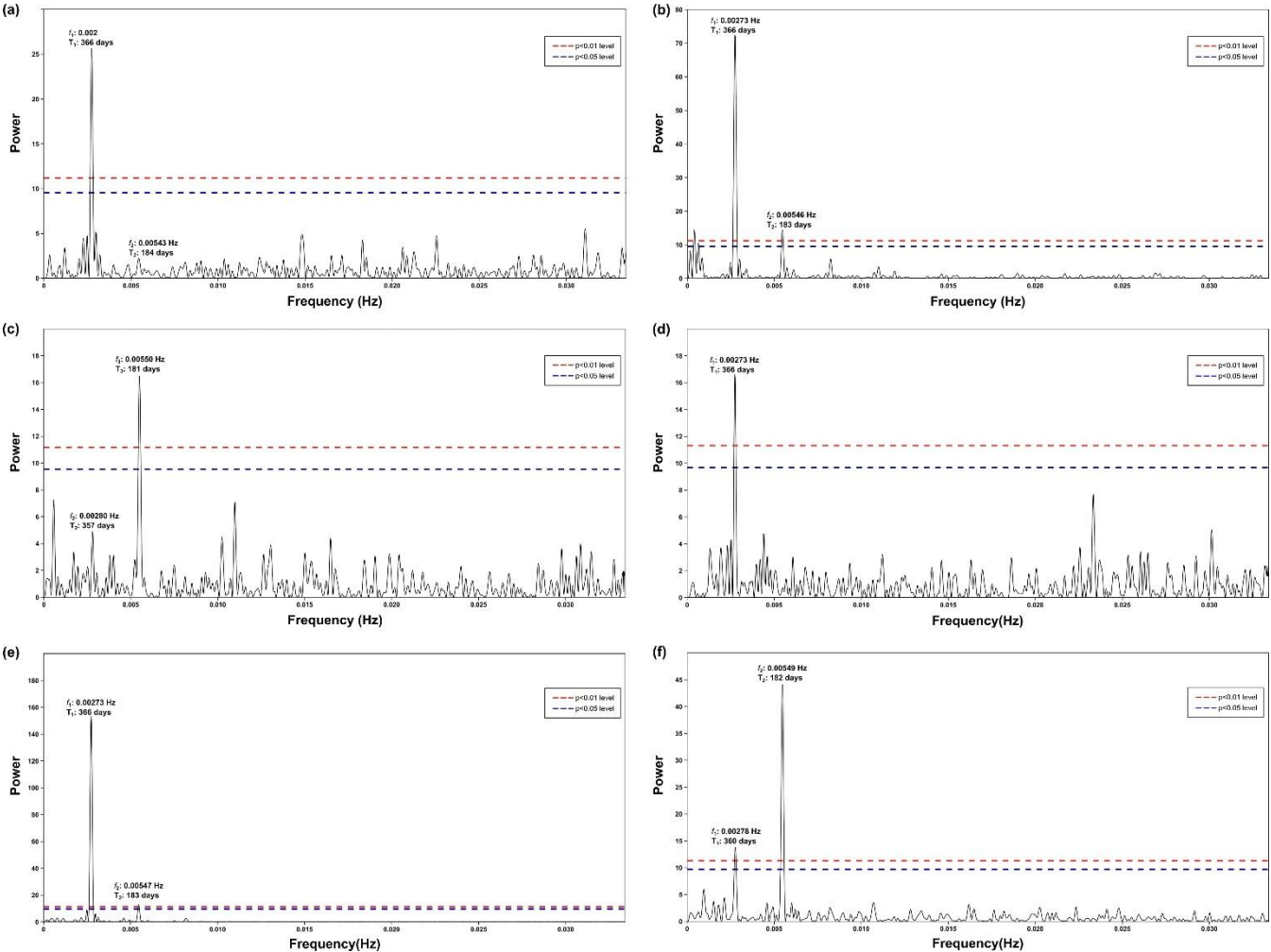
835 Figure A3: Periodogram of spectral analysis in time series of (a) surface wind speed, (b) surface wind direction, (c) frequency of dust storm events observed at the Nouadhibou airport, (d) aerosol dust concentration (aerosol optical depth) observed in Cabo Verde by NASA AERONET satellite, (e) sea surface temperature, and (f) upwelling index.
