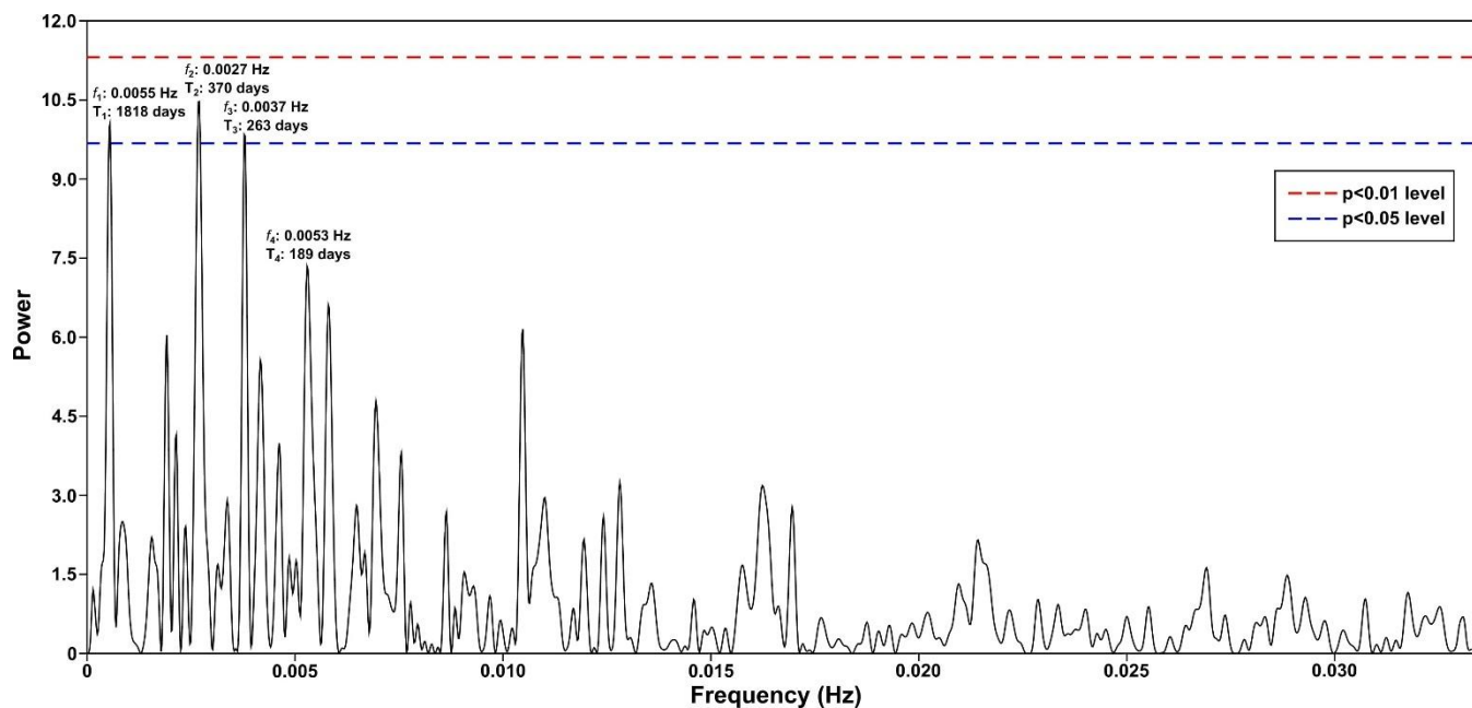
825 Figure A1: Periodogram of spectral analysis applied to the time series of total dinocysts export flux. This graph depicts the four highest frequencies ( f ) equivalent to periods ( T ) that occurred in the wavelet power spectra, of which three periodicities cross the significance line ( p < 0.05 ).
