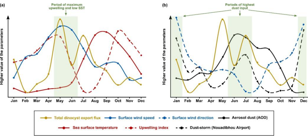
Figure 7: The comparison of monthly average data of total dinocyst export flux time series (yellow lines) from 2003 until 2020 with the environmental parameters showcasing (a) the dinocyst export flux peak in spring coincided with the highest upwelling intensity, and (b) the dinocyst export flux peaks in winter and summer coincided with the highest intensity of dust input.
