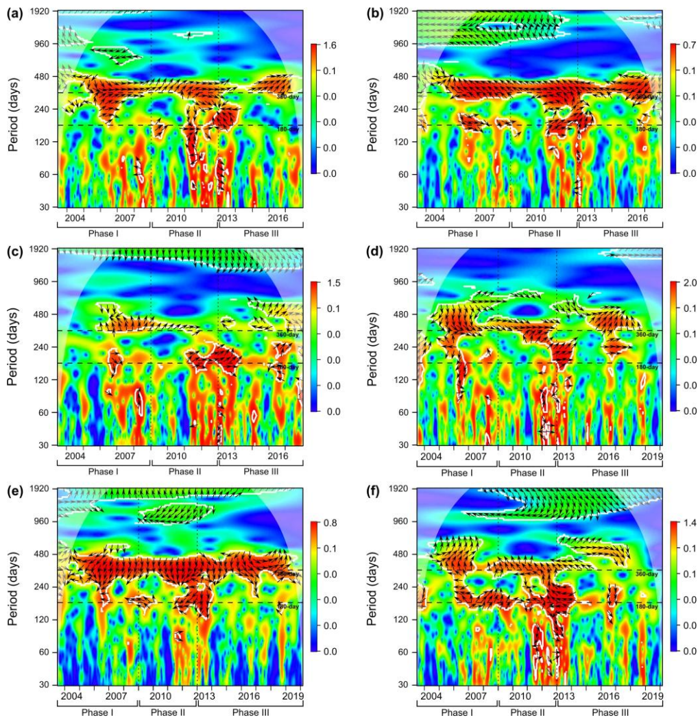
Figure 8: The wavelet cross-correlation analyses between time series of environmental parameters ( z_1 ): (a) surface wind speed, (b) surface wind direction, (c) dust storm events (Nouadhibou airport), (d) aerosol dust concentration (Cabo Verde), (e) sea surface temperature, (f) upwelling index; and total dinocyst export flux ( z_2 ). The colours of wavelet spectra indicate correlation level, white solid lines represent lines of significance, transparent grey area marks the cone of influence, vertical dashed lines indicate phase separation, and the black
