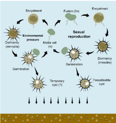
Figure 1: The simplified scheme of dinoflagellate cysts formation (encystment) shows two types of cysts: fossilisable cysts through sexual
