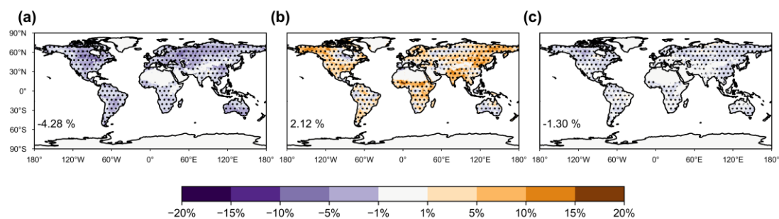
Figure 7. The same as Figure 6 but GLENS is applied. Results shown are the changes in frequency of drought extremes (scPDSI < -4) under SAI scenarios relative to RCP8.5 at 2075-2094 attributable to (a) temperature, (b) precipitation, and (c) radiation changes.
