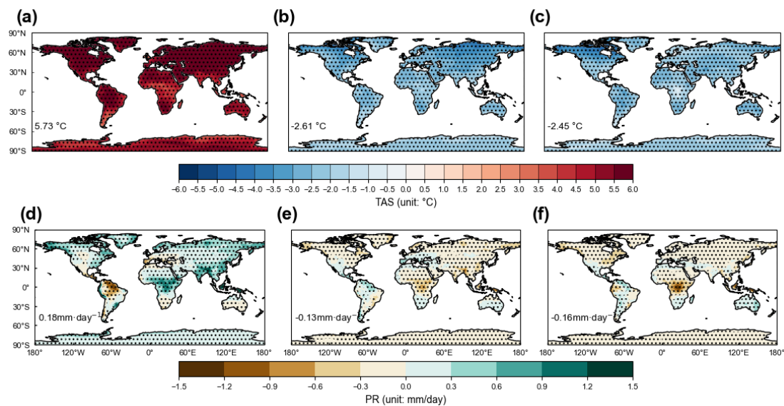
815 Figure 2. Climatic responses to global warming and SRM in GeoMIP. Results 816 shown are the spatial pattern of annual mean changes in (a, b, c) surface air temperature 817 (TAS) and (d, e, f) precipitation (PR) at 2081-2100 under (a, d) SSP5-8.5 scenario 818 relative to the historical period of 1995-2014, as well as that under (b, e) G6solar and 819 (c, f) G6sulfur scenarios relative to SSP5-8.5 both at 2081-2100. The dotted areas 820 indicate regions where at least four out of five models show changes with the same 821 signs. The mean value of the difference over global land surface is shown at the lower- 822 left of each panel.
