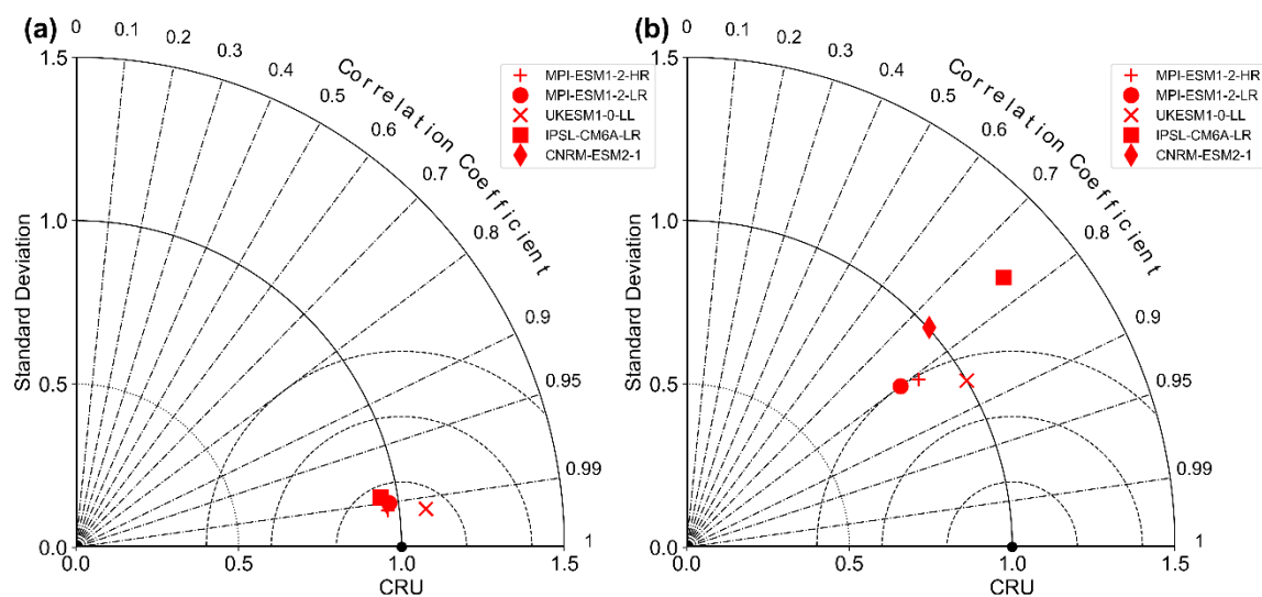
809 Figure 1. Evaluation of climate models from GeoMIP6. Results shown are the Taylor 810 diagram of annual mean (a) temperature and (b) precipitation for GeoMIP6 models 811 during the period of 1995–2014.
