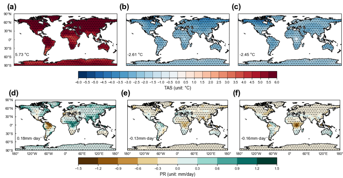
818 Figure 2. Climatic responses to global warming and SRM in GeoMIP. Results 819 shown are the spatial pattern of annual mean changes in (a, b, c) surface air temperature 820 (TAS) and (d, e, f) precipitation (PR) at 2081-2100 under (a, d) SSP5-8.5 scenario 821 relative to the historical period of 1995-2014, as well as that under (b, e) G6solar and 822 (c, f) G6sulfur scenarios relative to SSP5-8.5 both at 2081-2100. The dotted areas 823 indicate regions where at least four out of five models show changes with the same 824 signs. The mean value of the difference over global land surface is shown at the lower- 825 left of each panel.
