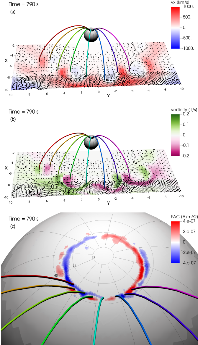
Figure 7. The coupling of magnetic field lines to the ionospheric grid. Panel (a) shows the velocity x -component in the current sheet ( B_x = 0 ). The arrows point to the direction of the plasma velocity in the current sheet. The colouring of the traced field lines has no physical meaning. The axes units are in R_E . Panel (b) shows via the colormap the vorticity of bulk flow (\nabla \times \mathbf{V})_z on the current sheet. Panel (c) is a zoomed-in section of the ionospheric grid, where the same field lines as in panels (a) and (b) can be seen to map to the ionosphere. Here the colormap shows FAC strength.
