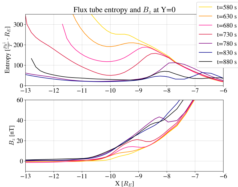
Figure 5. The radial profiles of flux tube entropy and B_z at Y=0 . The flux tube entropy is calculated along closed magnetic field lines. Note that the resolution of the simulation changes at \sim -8R_E , Earthward of this point the resolution is lower.
