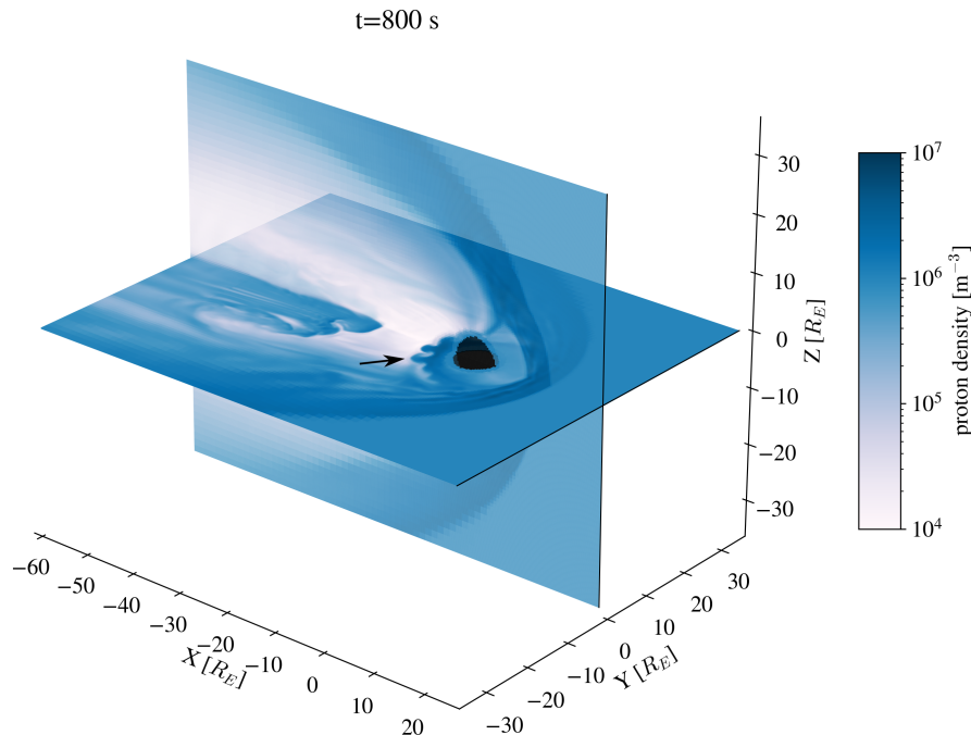
Figure 1. Part of the Vlasior simulation domain, Y=0 and Z=0 planes, the axes are given in R_E . The colours show the proton density in the solar wind and magnetosphere at t = 800 s. The simulation used GSE coordinates, with positive X directed towards the Sun. The solar wind enters the simulation box from the +X boundary, and flows in the -X direction. The vortex structure studied in this paper is indicated with an arrow on the nightside.
