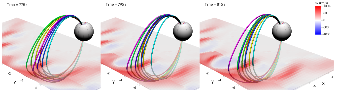
Figure 6. A zoomed in section of the magnetotail, where we trace selected field lines on the current sheet plane as the simulation progresses. The colours are used to distinguish the field lines from each other. The colormap shows the x-component of velocity in the magnetotail current sheet (where B_x=0 ). The axes are in R_E .
