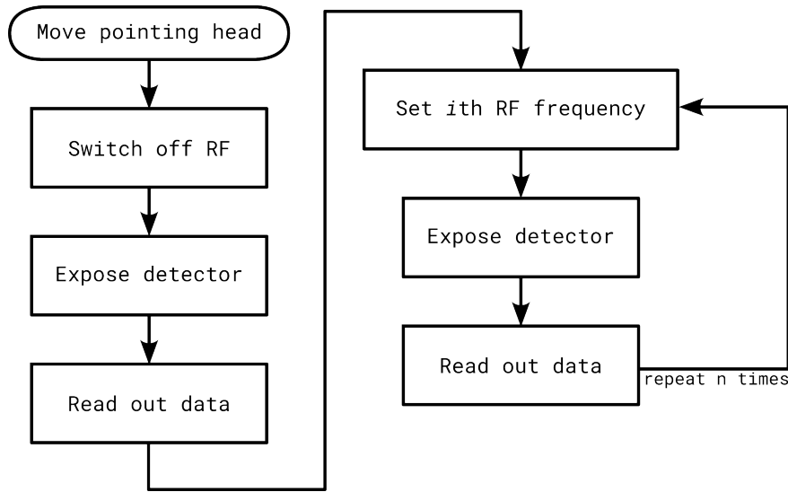
Figure 3. Schematic representation of the acquisition process for a single hypercube . For every acoustic frequency n , the corresponding RF frequency i needs to be set.
