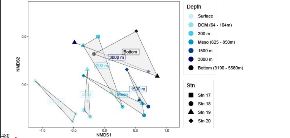
Figure 6: Non-metric multidimensional scaling (NMDS) plots based on Bray-Curtis dissimilarity shows bacterial communities clustered by depth. Stations are represented by shapes; depths are indicated by colors (see key). The grey shaded regions in the NMDS plots represent the clustering of bacterial communities by depth. Bacterial communities in subsurface waters differed substantially from their surface counterparts (ANOSIM, R-stat = 0.3248, p = 0.0052; Fig. 6; Suppl. Fig. 5). Stn. 17 bottom water (at 625 m) had a strong representation of Gammaproteobacteria (~35% of the community), while the contribution of Prochlorococcus and Alphaproteobacteria decreased relative to the surface and DCM. At Stn. 18, the communities at 300 m, the lower mesopelagic, and 1500 m were
