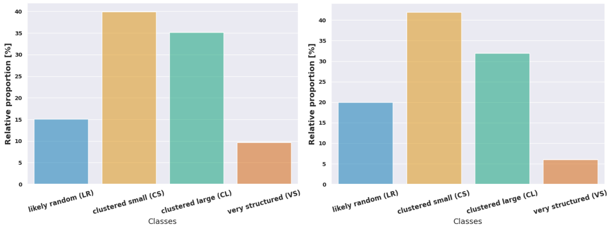
Figure S2: Histograms of the 4 classes population for Left: the TOOCAN-radar dataset, Right, the TOOCAN-RCE dataset
