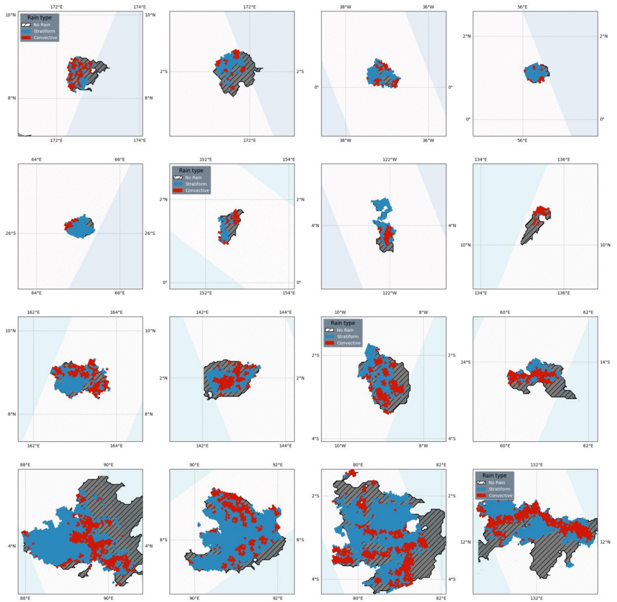
Figure S3: Same as Figure 1, 4 other examples for the 4 organizational classes by row from top to bottom: likely random (LR), small (CS), clustered large (CL), very structured scenes (VS)
