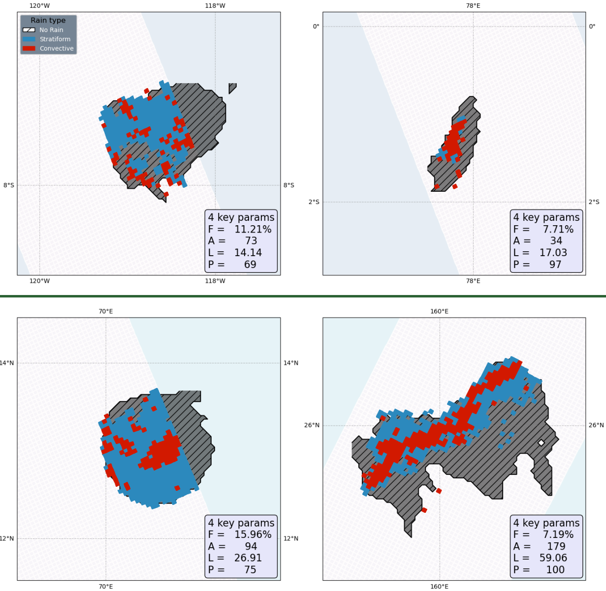
Figure 14: Same as figure 1. Archetypal examples of a) likely random (LR), b) clustered small (CS), c) clustered large (CL), d) very structured scenes (VS). The values of the four key parameters are indicated for each example.
