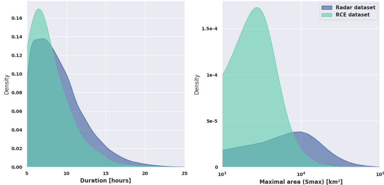
Figure 11: Empirical probability density function (estimated via KDE) of DCS properties from the scenes. Left: Duration in hour, Right: Maximum area in \text{km}^2 for the TOOCAN-radar dataset (dark blue) and the TOOCAN-RCE dataset (light blue).
