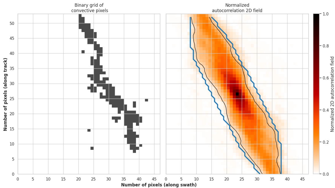
Figure S1: Same as Figure 2 for remaining selected scenes of Figure 14. Left: 2D binary scene (black pixels represent convective areas). Right: 2D autocorrelation normalized field, black contour shows the 10% contour and blue contour represents the convex contour that encompasses that 10% contour. The characteristic length L is the maximum distance between 2 points within the blue contour, here top: L \approx 18.44 , bottom: L \approx 14.14
