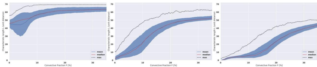
Figure B1: Same as figure 10 with Left: T=5\% threshold, Middle: T=10\% threshold, Right: T=15\% threshold for square clusters partition with MaxSquareSize \leq 3 .
