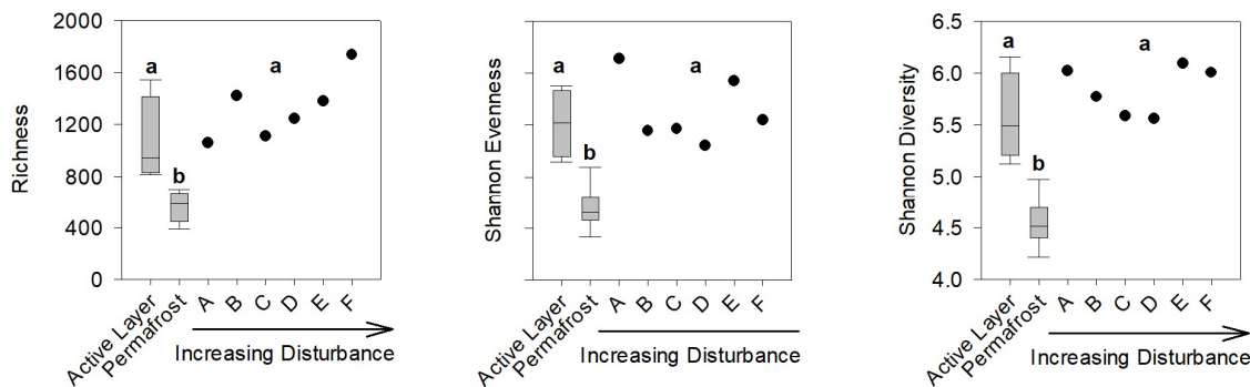
Figure 3: Microbial diversity in permafrost responds to abrupt thaw. Box and whisker plots of diversity metrics across active layer, permafrost, and disturbance gradient soils.
