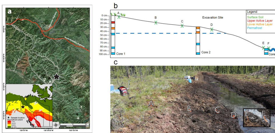
Figure 1: Dominion Creek core and surface sample locations. (a) Map of Dominion 120 Creek area and sampling site within Yukon Territory (Source: USGS & The Government of Canada). The map of the Dominion Creek region was assembled in ArcGIS 10.6.1. (b) Cross- section of disturbance gradient soils and permafrost cores. The horizontal line represents the
