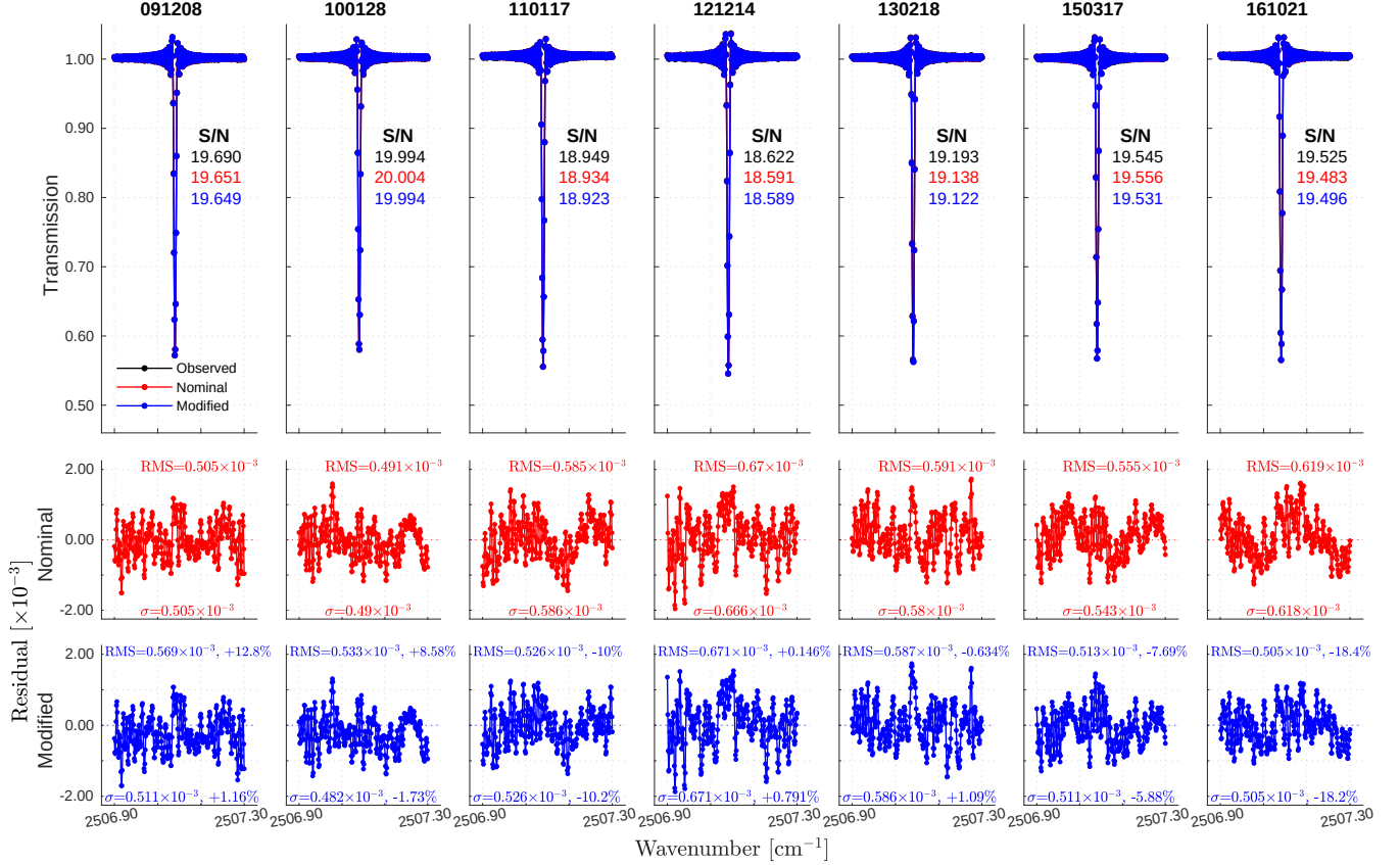
Figure 14. The top row shows the P(2) line of the HBr transmission spectrum, showcasing observed, fitted, and reconstructed spectra across different dates. The middle and bottom rows show residual plots comparing the deviations before and after fitting, respectively.
