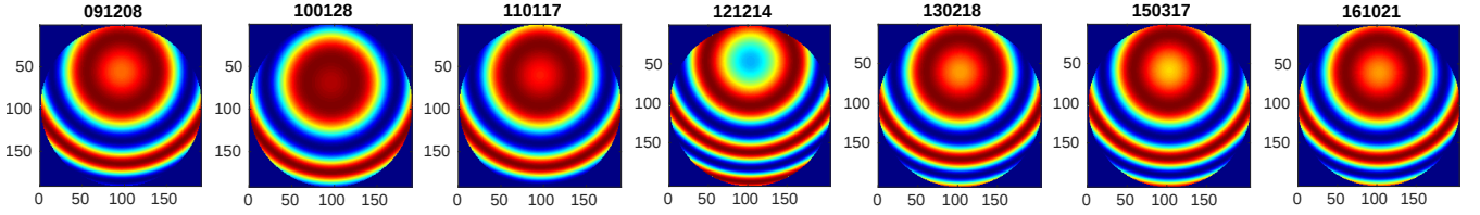
Figure 17. Haidinger fringe patterns near ZPD simulated under nominal configuration using ALIGN60 across multiple dates
