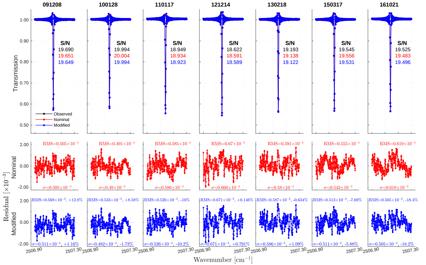
Figure 14. The top row shows the P(2) Isidelobe, fitted, and reconstructed spectra across different dates. The middle and bottom rows show residual plots comparing the deviations before and after fitting, respectively.
