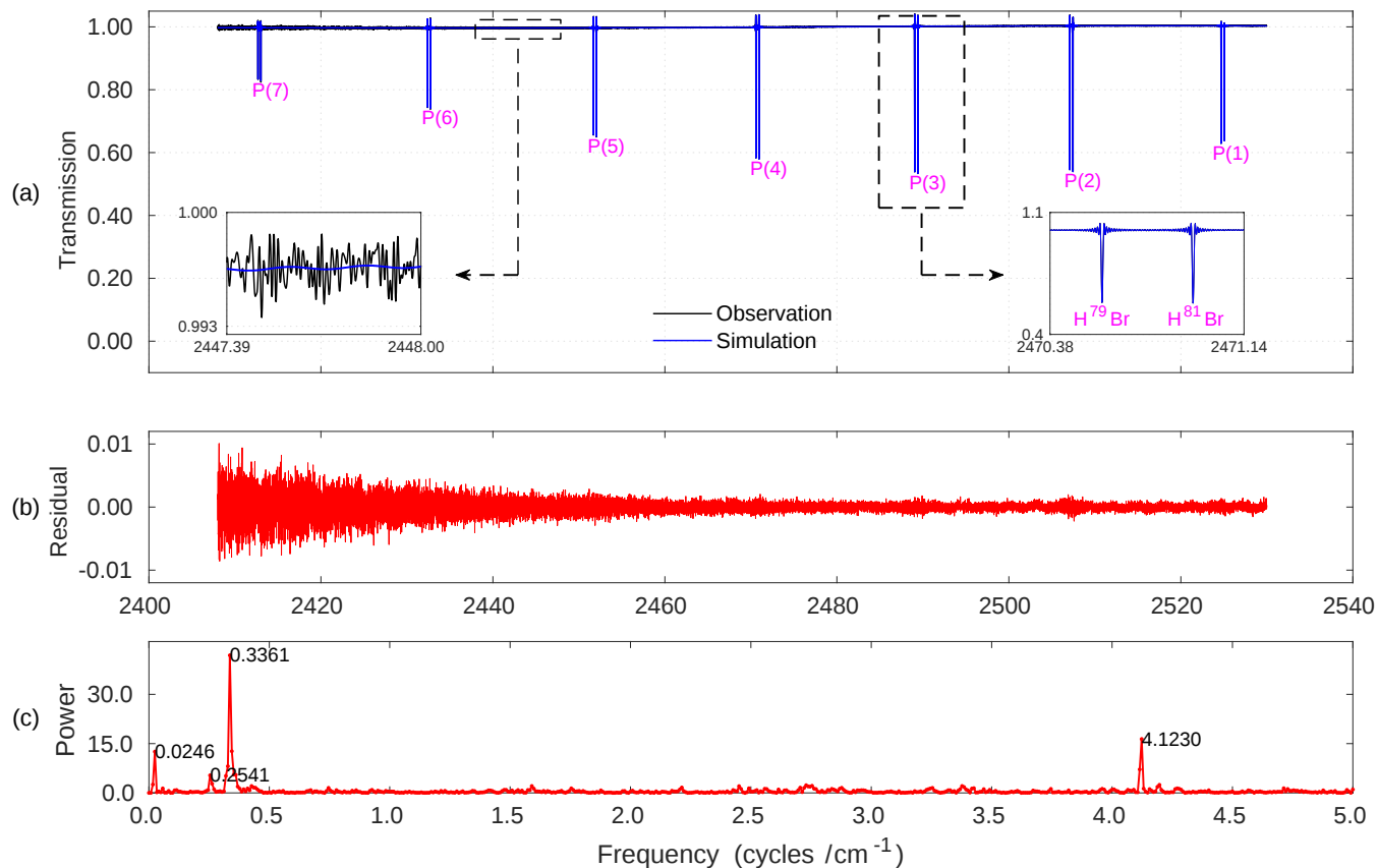
Figure 6. HBr transmission spectra acquired via gas cell measurement. (a) Comparison between observed and simulated spectra in the region 2400\text{--}2540\text{ cm}^{-1} , illustrating P-branch transitions. Insets display isotopic splitting (right) and low-amplitude channeling patterns (left). (b) Residuals between experiment and simulation. (c) FFT of the residual showing dominant frequencies linked to channeling artifacts arising from instrumental imperfections. Data acquired on December 14 th , 2012.
